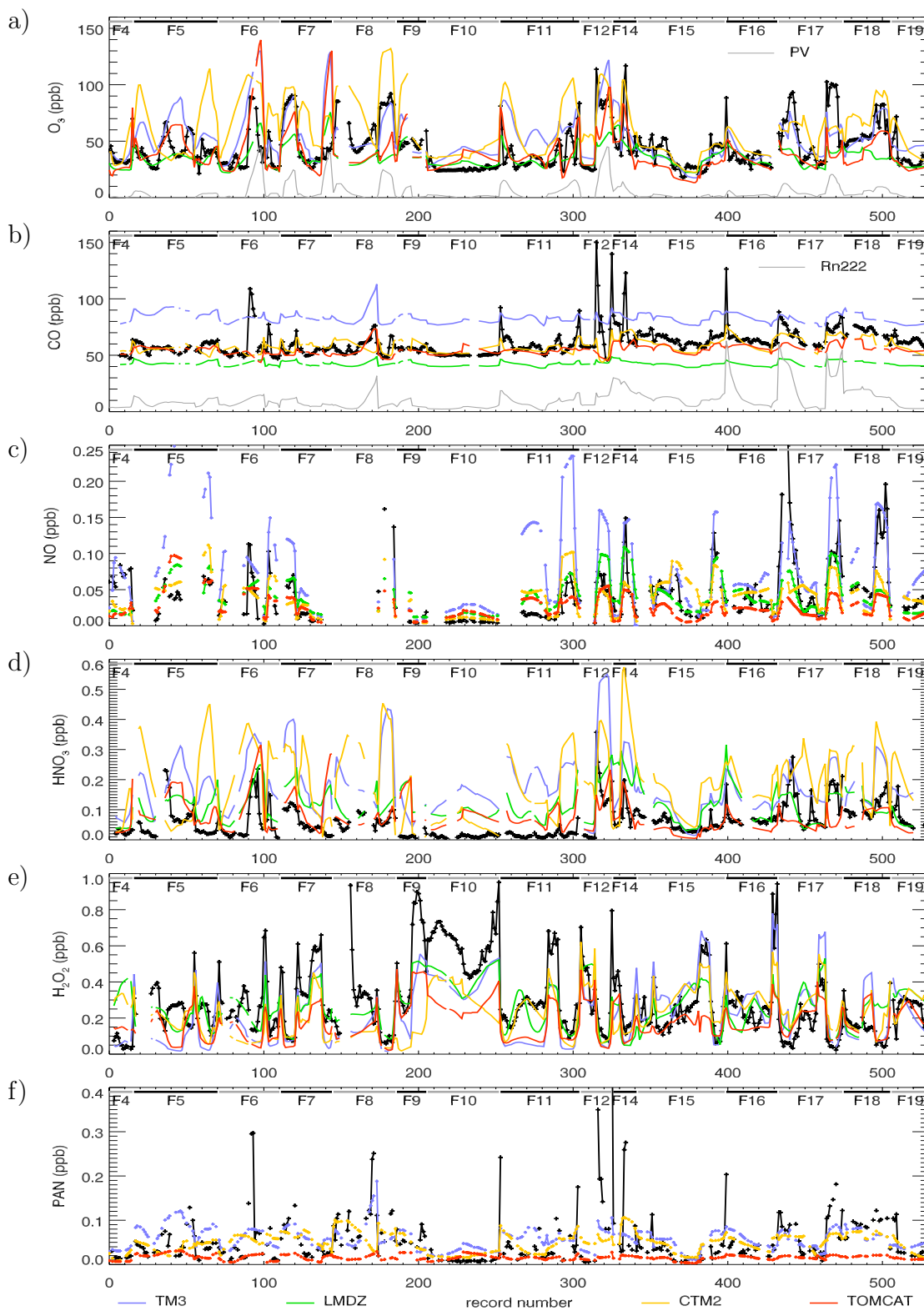
Fig. 2. Composites of PEM-Tropics A time series. Measurements at 0\text{--}35^\circ\text{S} and 400\text{--}200\text{ hPa} (about 7.2\text{--}12\text{ km} ) only. Flight numbers are indicated at the top of each panel. Black: measurements. Colors: simulations of the different models (see legend for color code). The grey line in the top panel a ) is potential vorticity (PVU) from the LMDz-INCA model, scaled by a factor of 10 to fit on the O_3 axis scale. Similarly, Rn222 (mol/1e22mol) is shown in grey in panel b ) and is displayed on the same y-axis as CO .
