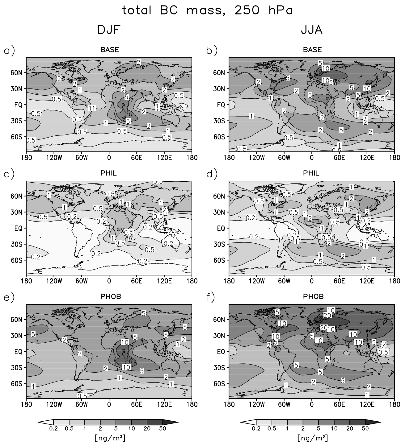
Fig. 4. Total BC mass concentration ( \text{ng/m}^3 ) at 250 hPa (main aircraft flight level) during northern hemispheric (NH) winter (left) and summer (right) simulated in the experiments BASE (a, b), PHIL (c, d) and PHOB (e, f). The results represent 4-year averages of the December to February and the June to August periods, respectively.
