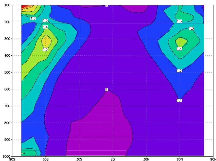
Fig. 12. Ratio of OH:HO 2 in scenario “high lat” to OH:HO 2 in scenario “no hal”. The numbers are zonally and annually averaged. The ordinate is the \sigma -level multiplied by 1000 which is approximately the pressure in hPa and the abscissa is latitude in degrees. Note that 24h averages are plotted.
