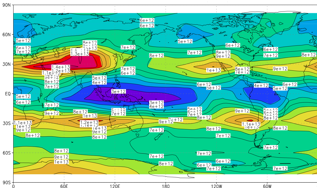
Fig. 7. Annually averaged tropospheric vertical column of BrO (in \text{molec cm}^{-2} ) for the scenario “high lat”. We used the WMO definition for the determination of the tropopause. Note that 24h averages are plotted. The ordinate is latitude in degrees and the abscissa is longitude in degrees.
