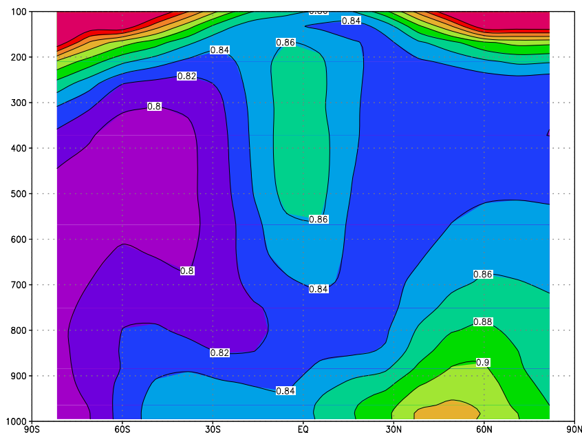
Fig. 10. Ratio of O_3 in scenario “tropics” to O_3 in scenario “no hal”. The numbers are zonally and annually averaged. The ordinate is the \sigma -level multiplied by 1000 which is approximately the pressure in hPa and the abscissa is latitude in degrees. Note that 24h averages are plotted.
