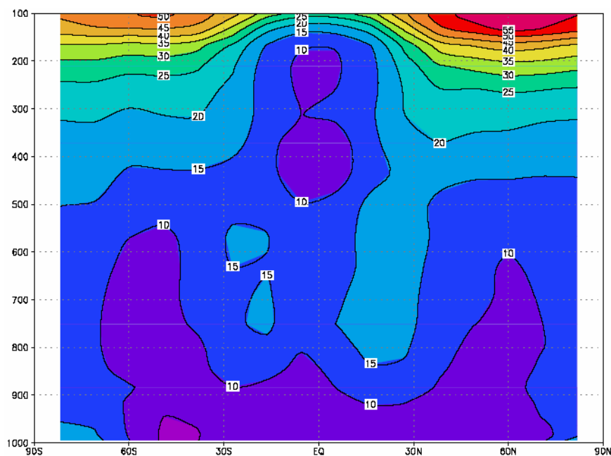
Fig. 3. Zonally and annually averaged mean of the lifetime of \text{Br}_{\text{inorg}} (in days) resulting from our source scenario “high lat”. The ordinate is the \sigma -level multiplied by 1000 which is approximately the pressure in hPa and the abscissa is latitude in degrees.
