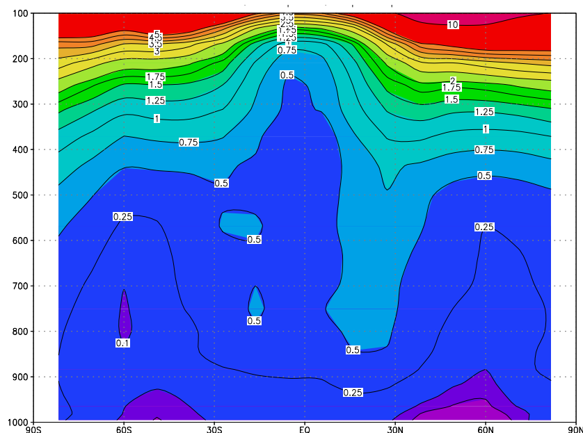
Fig. 5. Zonally and annually averaged mean of the BrO mixing ratio (in \text{pmol mol}^{-1} ) resulting from our source scenario “tropics”. The ordinate is the \sigma -level multiplied by 1000 which is approximately the pressure in hPa and the abscissa is latitude in degrees. Note that 24h averages are plotted. Seasalt aerosol is not explicitly included as a source therefore boundary layer values are lower limits.
