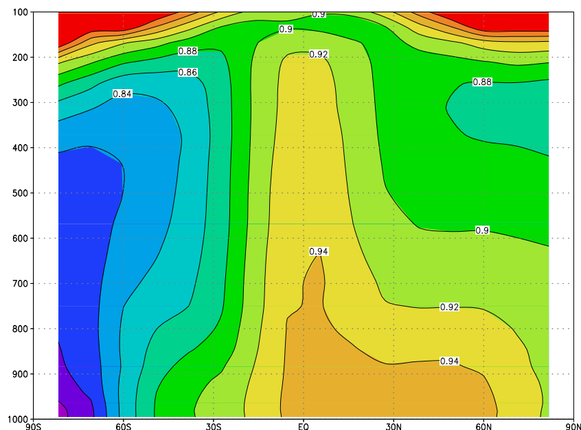
Fig. 9. Ratio of O_3 in scenario “high lat” to O_3 in scenario “no hal”. The numbers are zonally and annually averaged. The ordinate is the \sigma -level multiplied by 1000 which is approximately the pressure in hPa and the abscissa is latitude in degrees. Note that 24h averages are plotted.
