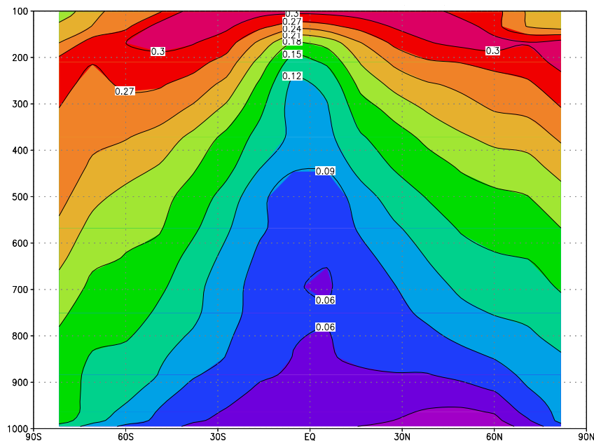
Fig. 2. Zonally and annually averaged mean of the ratio of \text{BrO} to \text{Br}_{\text{inorg}} resulting from our source scenario “high lat”. The ordinate is the \sigma -level multiplied by 1000 which is approximately the pressure in hPa and the abscissa is latitude in degrees. Note that 24h averages are plotted.
