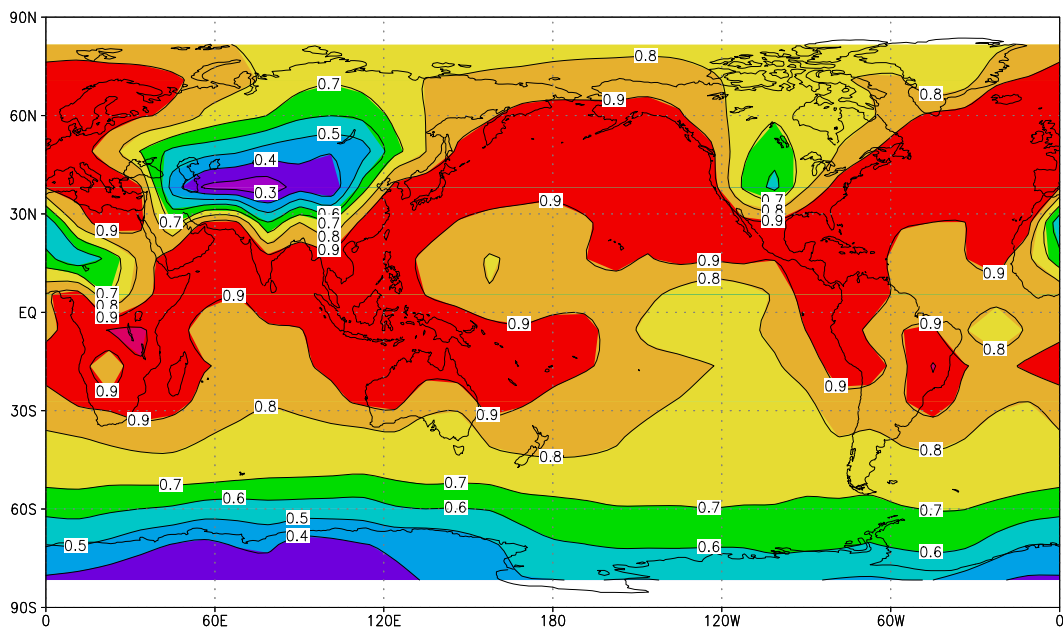
Fig. 16. Ratio of the vertical column of DMS for the scenario “tropics” to scenario “no hal” (annually averaged). The ordinate is latitude in degrees and the abscissa is longitude in degrees. Seasalt aerosol is not explicitly included as a source for BrO therefore the reductions in DMS are lower limits.
