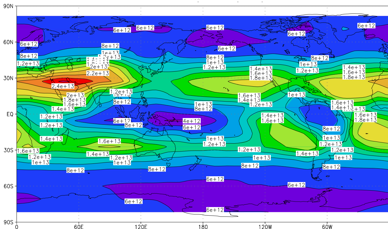
Fig. 8. Annually averaged tropospheric vertical column of BrO (in \text{molec cm}^{-2} ) for the scenario “tropics”. We used the WMO definition for the determination of the tropopause. Note that 24h averages are plotted. The ordinate is latitude in degrees and the abscissa is longitude in degrees.
