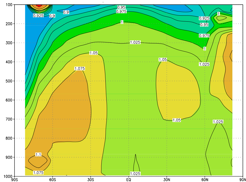
Fig. 14. Ratio of \text{NO}:\text{NO}_2 in scenario “high lat” to \text{NO}:\text{NO}_2 in scenario “no hal”. The numbers are zonally and annually averaged. The ordinate is the \sigma -level multiplied by 1000 which is approximately the pressure in hPa and the abscissa is latitude in degrees. Note that 24 h averages are plotted.
