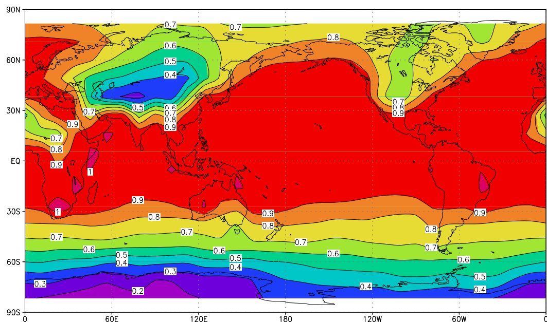
Fig. 15. Ratio of the vertical column of DMS for the scenario “high lat” to scenario “no hal” (annually averaged). The ordinate is latitude in degrees and the abscissa is longitude in degrees. Seasalt aerosol is not explicitly included as a source for BrO therefore the reductions in DMS are lower limits.
