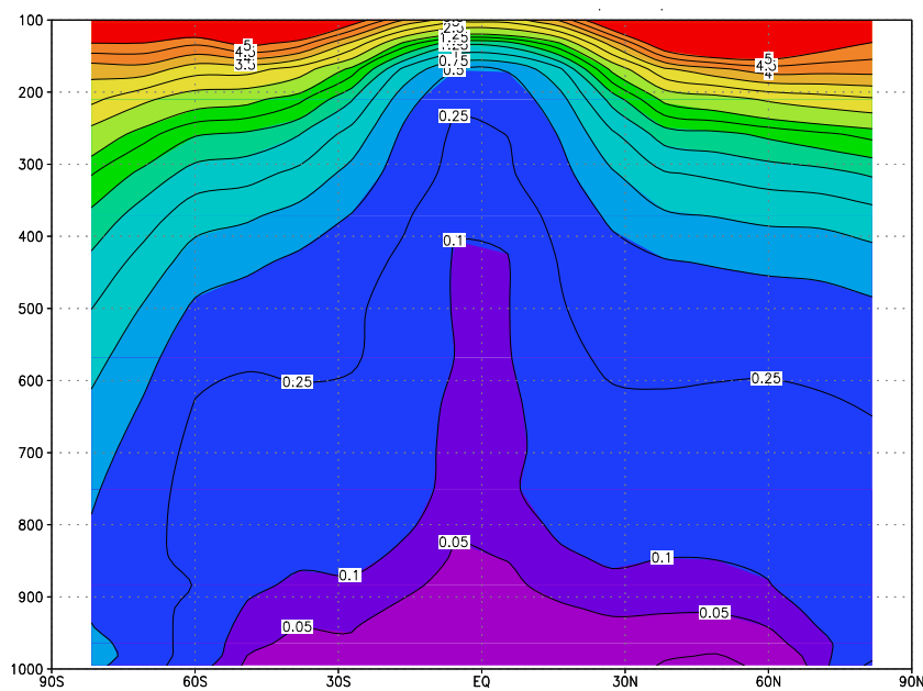
Fig. 4. Zonally and annually averaged mean of the BrO mixing ratio (in \text{pmol mol}^{-1} ) resulting from our source scenario “high lat”. The ordinate is the \sigma -level multiplied by 1000 which is approximately the pressure in hPa and the abscissa is latitude in degrees. Note that 24h averages are plotted. Seasalt aerosol is not explicitly included as a source therefore boundary layer values are lower limits.
