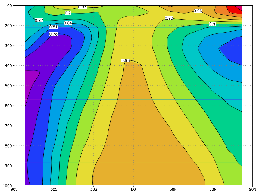
Fig. 13. Ratio of \text{H}_2\text{O}_2 in scenario “high lat” to \text{H}_2\text{O}_2 in scenario “no hal”. The numbers are zonally and annually averaged. The ordinate is the \sigma -level multiplied by 1000 which is approximately the pressure in hPa and the abscissa is latitude in degrees. Note that 24 h averages are plotted.
