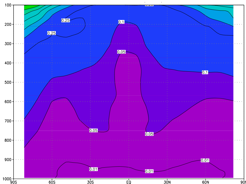
Fig. 6. Zonally and annually averaged mean of the BrO mixing ratio (in \text{pmol mol}^{-1} ) resulting from our source scenario “strat”. The ordinate is the \sigma -level multiplied by 1000 which is approximately the pressure in hPa and the abscissa is latitude in degrees. Note that 24h averages are plotted.
