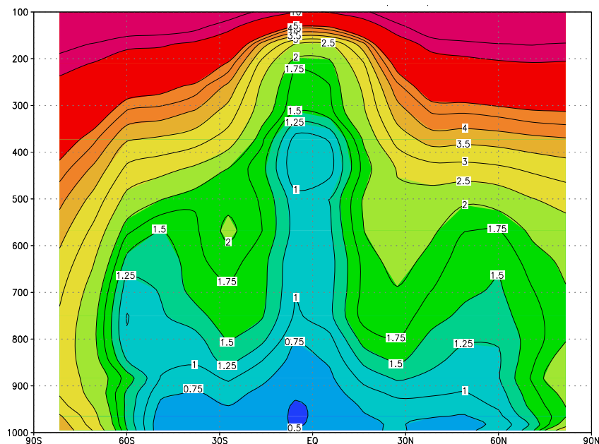
Fig. 1. Zonally and annually averaged mean of the \text{Br}_{\text{inorg}} mixing ratio (in \text{pmol mol}^{-1} ) resulting from our source scenario “high lat”. The ordinate is the \sigma -level multiplied by 1000 which is approximately the pressure in hPa and the abscissa is latitude in degrees. Note that 24h averages are plotted. Seasalt aerosol is not explicitly included as a source therefore boundary layer values are lower limits.
