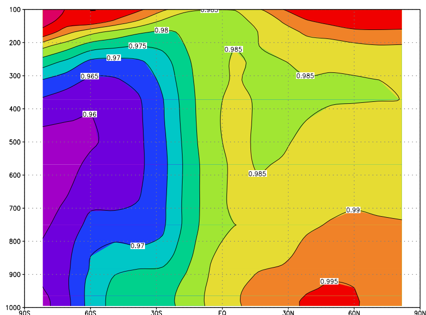
Fig. 11. Ratio of O 3 in scenario “strat” to O 3 in scenario “no hal”. The numbers are zonally and annually averaged. The ordinate is the \sigma -level multiplied by 1000 which is approximately the pressure in hPa and the abscissa is latitude in degrees. Note that 24 h averages are plotted.
