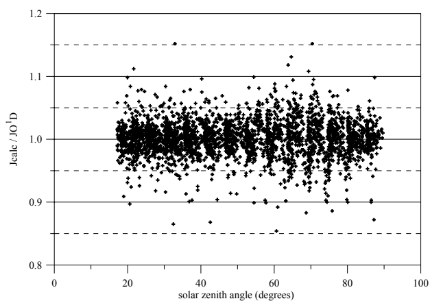
Fig. 7. Ratio of J_{calc} as a function of solar zenith angle from the Bentham's measurements data set. ( J_{calc} is calculated with method 2 using the global irradiance data and J(O^1D) using actinic flux spectra).
