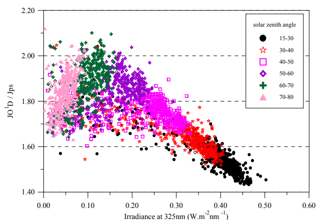
Fig. 6. Ratio of J(O 1 D)/ J_{ps} , as a function of global irradiance at 325 nm for different groups of solar zenith angles. (J(O 1 D)) was calculated from the spectral actinic flux data from the Bentham spectroradiometer and J_{ps} is calculated if the global irradiance is used instead of actinic flux in Eq. 1).
