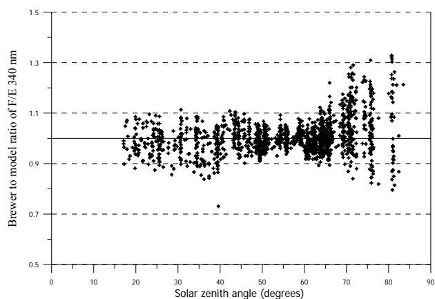
Fig. 5. Ratios of actinic to global irradiance at 340±2 nm as measured/retrieved from the Brewer and calculated with the TUV model. Measurements represent cloudless sky cases.
