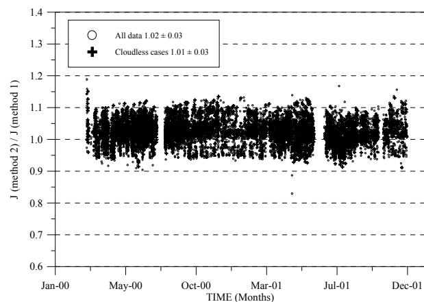
Fig. 10. Comparison of the ozone photolysis frequencies retrieved from the two methods described. J_{calc}/J_{rtv} ratio during the period February 2000–December 2001 calculated for Thessaloniki. Circles represent the full data set and crosses the cloudless sky cases.
