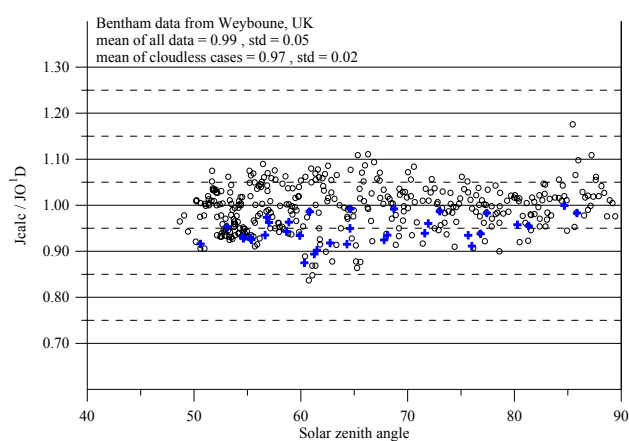
Fig. 9. Ratio of calculated J to J(O^1D) derived from global irradiance and actinic flux measurements from BENTHAM measurements at Weybourne, UK, as a function of solar zenith angle. Asterisks denote measurements under cloudless conditions.
