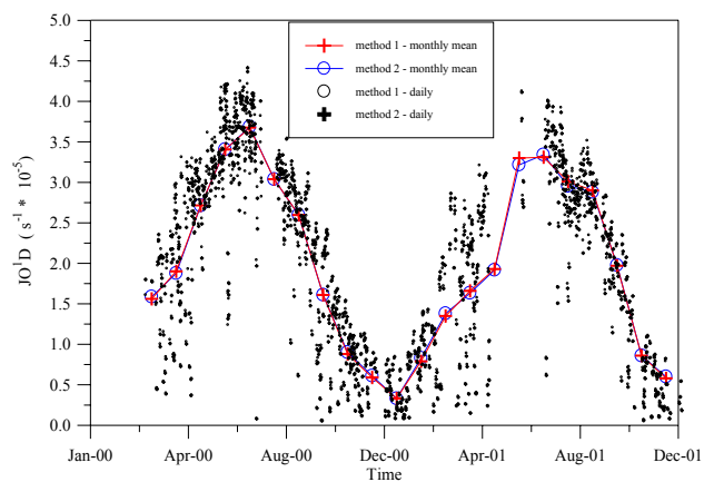
Fig. 11. Calculated JO 1 D during local noon for the period February 2000–December 2001, at Thessaloniki following the two retrieval methods. Monthly averages are also shown.
