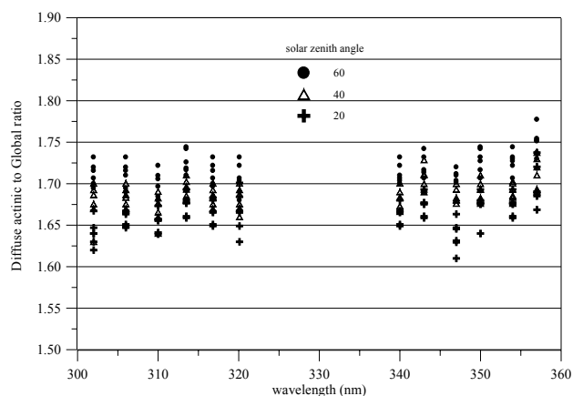
Fig. 1. Diffuse actinic flux to diffuse global irradiance [ A(\lambda) ] as a function of wavelength for three solar zenith angles, calculated from the integration of radiance measurements on cloudy-overcast conditions at Thessaloniki.
