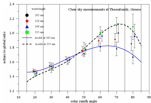
Fig. 3. Actinic to global ratio means for solar zenith angle groups of 10^\circ at 305 nm (circles), 320 nm (diamonds), 340 nm (triangles) and 355 nm (boxes). Model calculations at 305 nm (solid line) and 355 nm (dash line). All data represent cloudless sky measurements.
