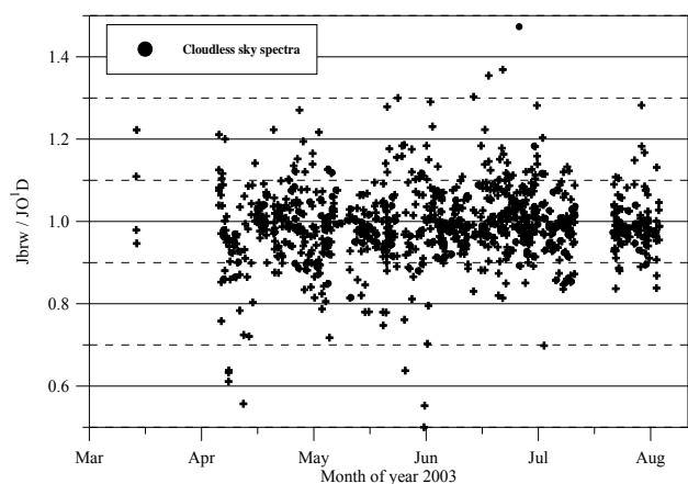
Fig. 8. \frac{J_{brw}}{J(O^1D)} ratio using global irradiance from Brewer MKIII. Circles represent measurements under cloudless sky conditions and crosses represent all measurements. ( J_{calc} is calculated with method 2 using the global irradiance data and J(O^1D) using actinic flux spectra from the Bentham instrument).
