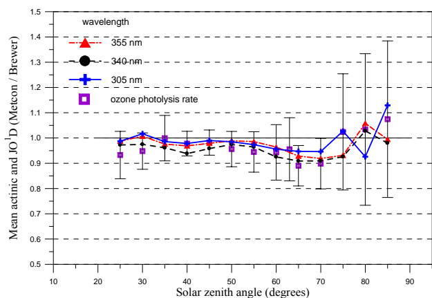
Fig. 4. Mean ratios of actinic fluxes measured by METCON and retrieved from the Brewer irradiances at 305±2 nm (crosses), 340±2 nm (circles), 355±2 nm (triangles) and of ozone photolysis frequencies (boxes), as a function of solar zenith angle (5° increments). The standard deviation for each solar zenith angle is shown only for 305 nm, representing the highest possible variability of the ratios.
