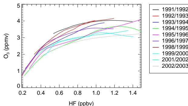
Fig. 5. Early winter reference relations for ten years from 1991–1992 to 2002–2003 are indicated as coloured lines. O 3 /HF is shown; HF being corrected for the growth rate of HF derived from the HALOE CH 4 /HF relationship for each year (Tilmes, 2003).
