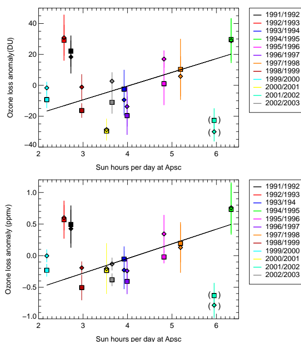
Fig. 17. Top panel: deviation of column ozone loss (DU) from the linear relation (black line in Fig. 16, top panel) in relation to sun hours per day at (A PSC ) (see text). Bottom panel: deviation of accumulated ozone loss in mixing ratio from the linear relation (black line in Fig. 16, bottom panel) in relation to sun hours per day at (A PSC ) (see text).
