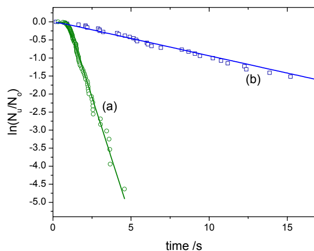
Fig. 2. Logarithm of the fraction of unfrozen droplets as a function of time after injection in the droplet levitator. (a) open circles: large droplets with an average radius r_1 = 49 \mu\text{m} , (b) open squares: small droplets with an average radius r_2 = 19 \mu\text{m} .
