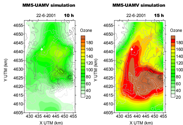
Fig. 3. Spatial distribution of ozone from UAMV simulation on 22 June, left panel at 10 h UTC and right panel at 15 h UTC. The colour ozone scale is in \mu\text{g m}^{-3} and the white rhombus show Vic location.
