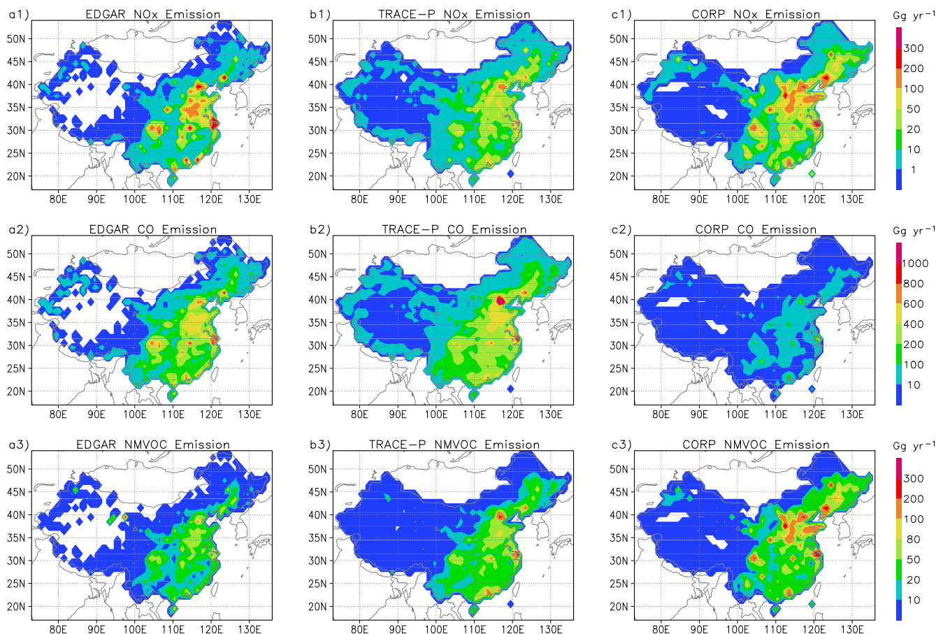
Fig. 1. Anthropogenic surface emissions of \text{NO}_x , CO, NMVOC over China according to the EDGAR, TRACE-P and CORP estimates. Both EDGAR and CORP estimates are for the year of 1995, and TRACE-P is for the year of 2000. While EDGAR and TRACE-P NMVOC emissions are independent on \text{NO}_x emissions, CORP NMVOC emissions are scaled to \text{NO}_x emissions. Units are \text{Gg yr}^{-1} per 1^\circ \times 1^\circ grid.
