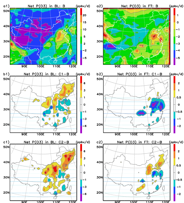
Fig. 3. Differences in calculated net production of ozone, P(\text{O}_3) , for the boundary layer (BL) and the free troposphere (FT) due to the use of different emission inventories EDGAR, TRACE-P and CORP (denoted as cases B, C1 and C2, respectively). Simulated results with EDGAR are given as reference and the differences are shown with the deviations of TRACE-P and CORP to EDGAR.
