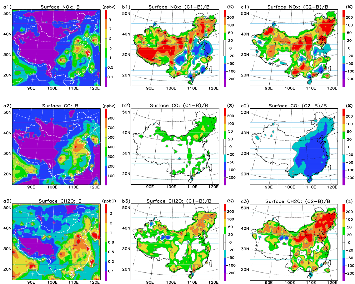
Fig. 2. Difference in surface \text{NO}_x , CO and \text{CH}_2\text{O} due to the use of different emission inventories EDGAR, TRACE-P and CORP (denoted as cases B, C1 and C2, respectively). Simulated results with EDGAR are given as reference and the differences are shown with the relative deviations of TRACE-P and CORP to EDGAR. Note that the relative differences are large for \text{NO}_x in western China due to low emissions and concentrations of \text{NO}_x in unpolluted areas.
