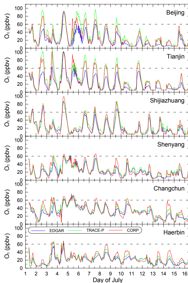
Fig. 7. Simulated hourly variations of surface \text{O}_3 for the selected model grid cells with different emission inventories EDGAR, TRACE-P and CORP (denoted as blue, green and red lines, respectively). The grid cells are denoted with the name of big cities which are included in the grid cells. The first-level ozone standard (60 ppbv) is shown with black dashed lines.
