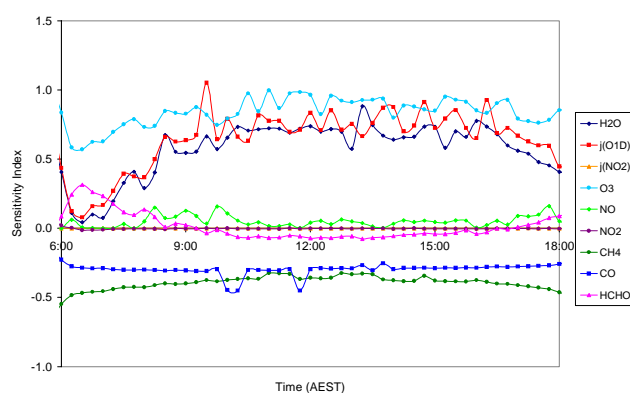
Fig. 9. Local Sensitivity Analysis of OH between 06:00 and 18:00 (7 February).
