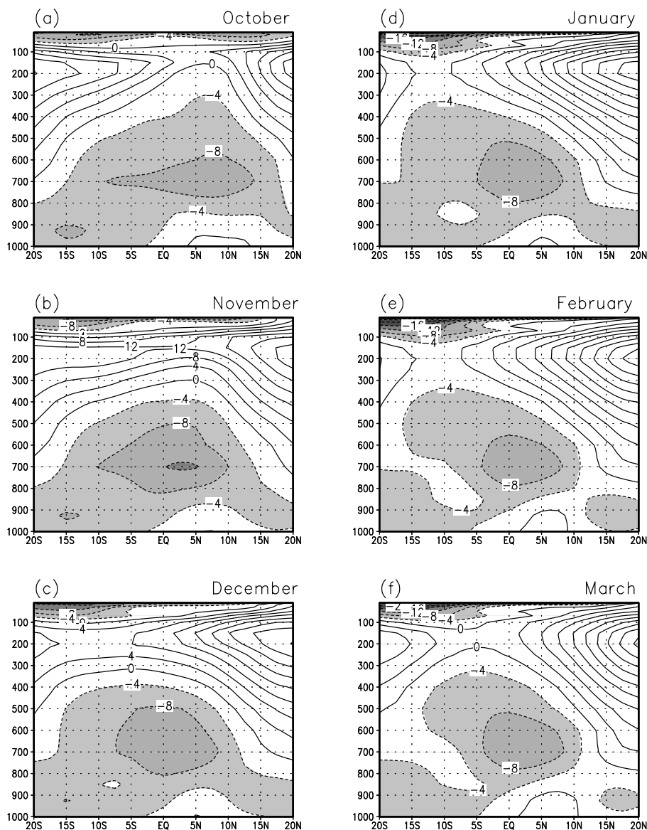
Fig. 9. Vertical Cross section of the climatological zonal wind at 10^{\circ} W for (a) October through (f) March. Units are \text{m}\cdot\text{s}^{-1} .
