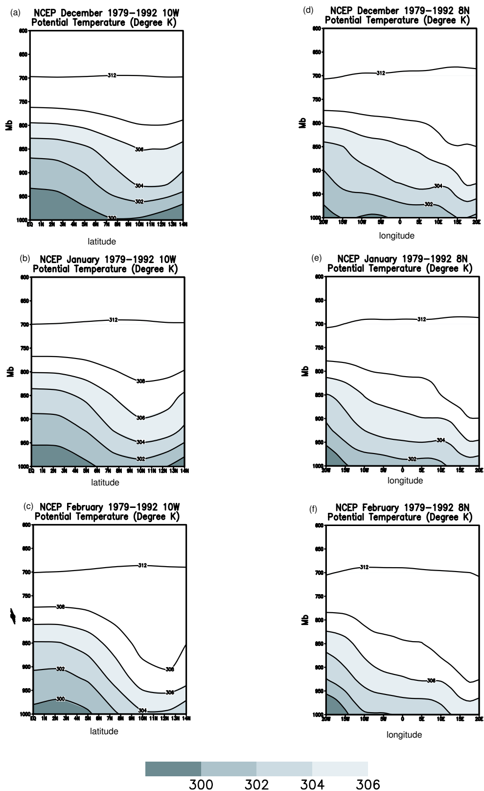
Fig. 12. NCEP 1000–600 hPa vertical cross section of Potential Temperatures at 10° W for (a) December, (b) January, (c) February and at 8° N (d) December, (e) January, (f) February. Units are degree K.
