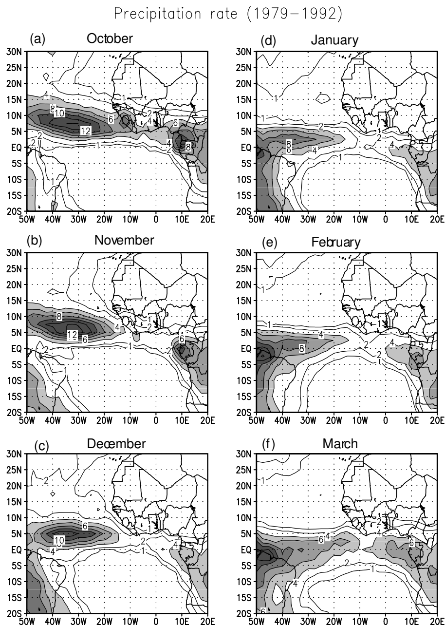
Fig. 11. The climatology of the precipitation rate for (a) October through (f) March averaged from 1979 to 1992. Units are \text{mm}\cdot\text{day}^{-1} .
