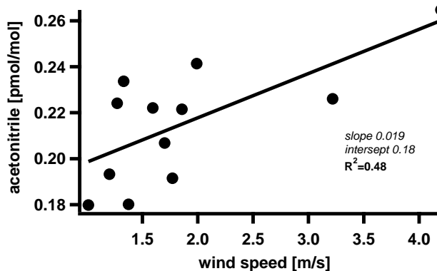
Fig. 3. Average daytime acetonitrile levels (11:00–16:00) versus average wind speeds.
