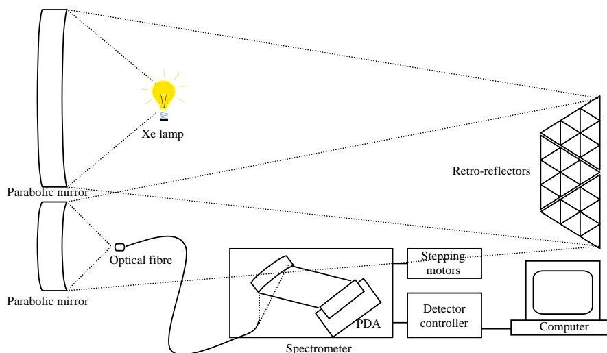
Fig. 2. Sketch of the long path DOAS system.
