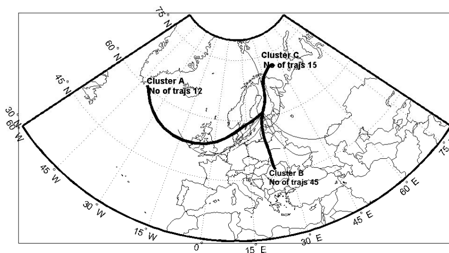
Fig. 14. Representation of trajectory clusters arriving Hyttiälä for the period Sep–Nov. The clusters are here presented as the mean of the trajectories building the clusters. Numbers of trajectories in cluster are also indicated.
