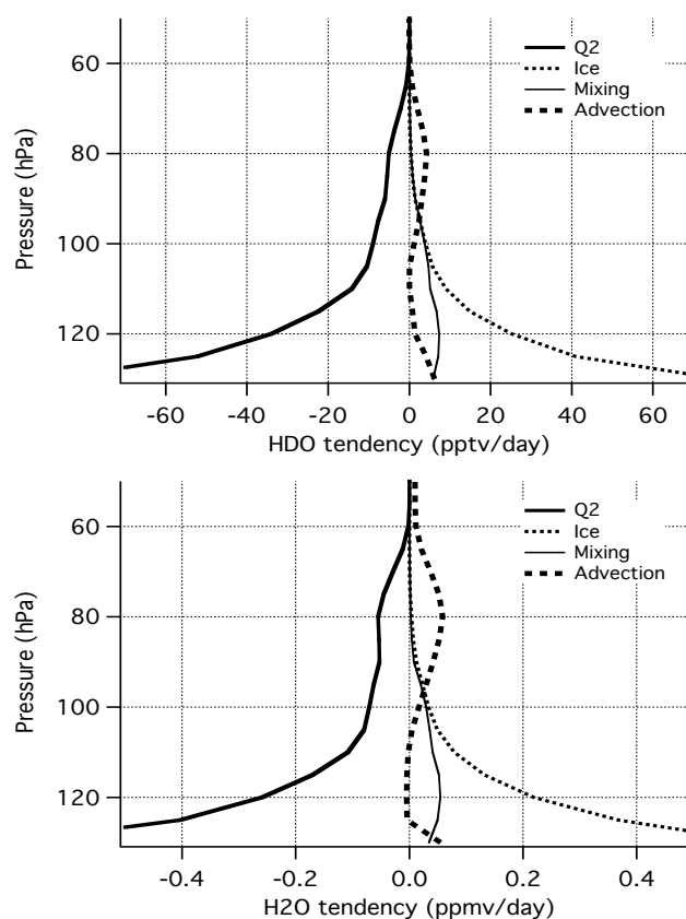
Fig. 5. Budget for HDO (top) and H_2O (bottom) in the TTL for \delta D_{ice} from the -565\% run, averaged over the model’s two regions. See the text for the definitions of the lines.
