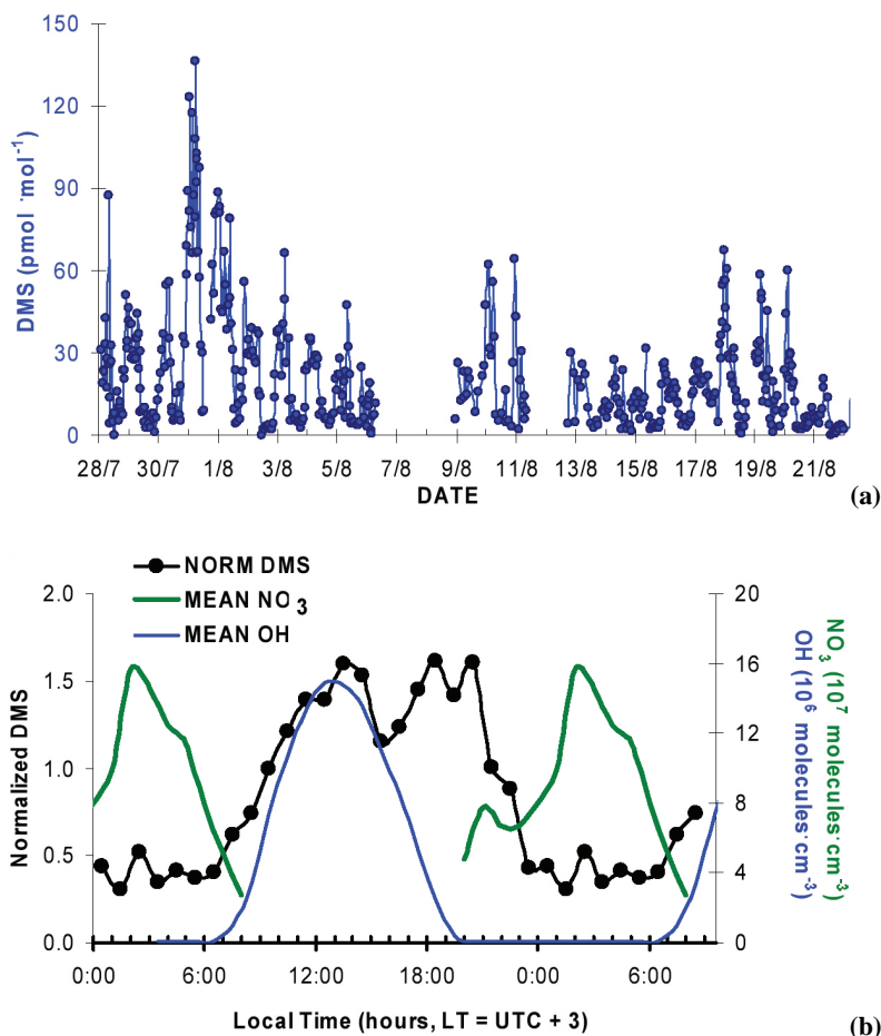
Fig. 2. Atmospheric concentrations of (a) DMS during the campaign and (b) diurnal variation of normalized DMS (Normalized DMS = \text{DMS}_{(\text{time } y, \text{day } x)} / \text{mean DMS}_{(\text{day } x)} ) in relation to the mean OH and \text{NO}_3 levels measured during the campaign. Time refers to local time (LT = UTC + 3)
