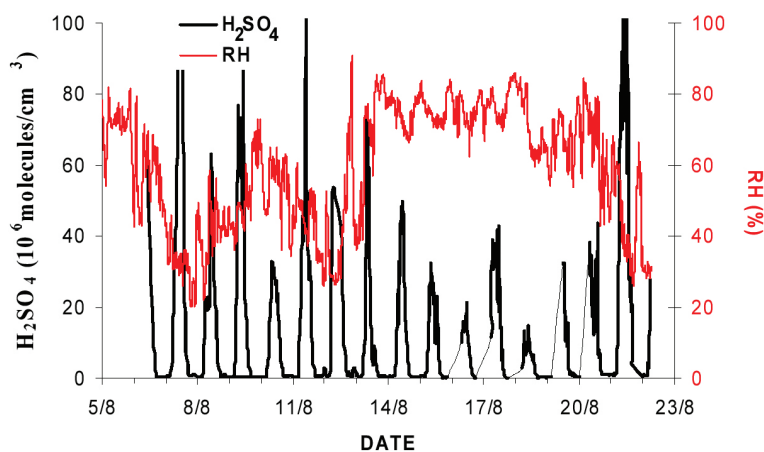
Fig. 6. Variation of atmospheric molecular concentrations of \text{H}_2\text{SO}_4 and RH during the campaign.
