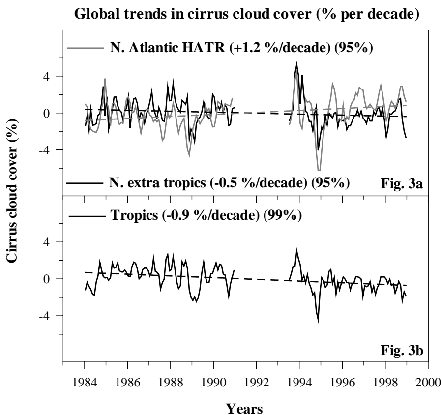
Fig. 3. (a) Trends in (CCC) (% per decade) for the period 1984–1998 over the northern extra tropics ( 30^{\circ}\text{N} – 70^{\circ}\text{N} , 180^{\circ}\text{W} – 180^{\circ}\text{E} ) and the North Atlantic high air traffic region ( 40^{\circ}\text{N} – 60^{\circ}\text{N} , 35^{\circ}\text{W} – 60^{\circ}\text{W} ). (b) Same as (a) but for the tropics ( 30^{\circ}\text{S} – 30^{\circ}\text{N} , 180^{\circ}\text{W} – 180^{\circ}\text{E} ).
