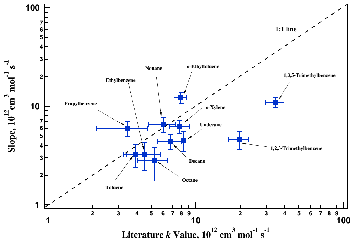
Fig. 4. Comparison of slopes of the \ln[X] - \sum[\text{OH}]t correlation lines for different components with literature k values. The horizontal bars represent the reported errors in the k values. The vertical bars are the standard deviations of the slopes.
