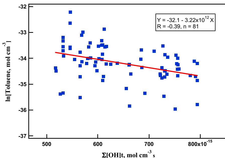
Fig. 3. Relationship between the mixing ratio of toluene and the integral of OH abundance over a 24 hour period prior to hydrocarbon measurement. Note that ln[Toluene] is used instead of [Toluene] and that the units are chosen so that the slope of the regression line can be compared with the OH rate constant k in cm 3 mol -1 s -1 . Correlation results for other hydrocarbons are summarized in Table 2.
