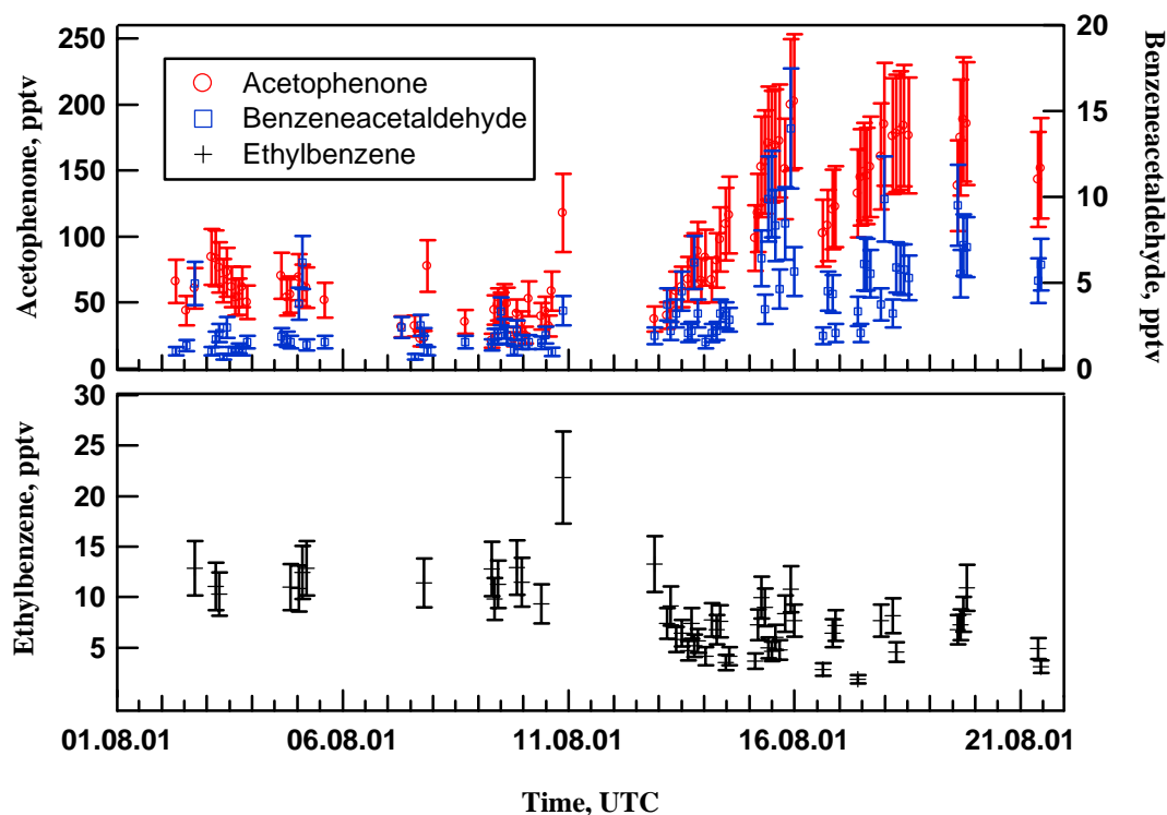
Fig. 5. Time series of ethylbenzene (bottom), acetophenone and benzeneacetaldehyde (top). The vertical bars represent the estimated errors.
