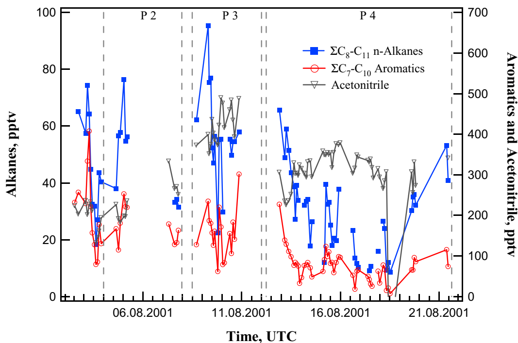
Fig. 1. Summed mixing ratios of C 8 –C 11 n-alkanes and C 7 –C 10 aromatics during the MINOS campaign. For the purpose of comparison average mixing ratios of acetonitrile derived from the PTR-MS measurements (Salisbury et al., 2003) are also shown. Due to interferences, 1,2,4-trimethylbenzene is not included in the mixing ratio of aromatics. The vertical dashed lines show the starts and ends of periods 2–4 (see Salisbury et al., 2003).
