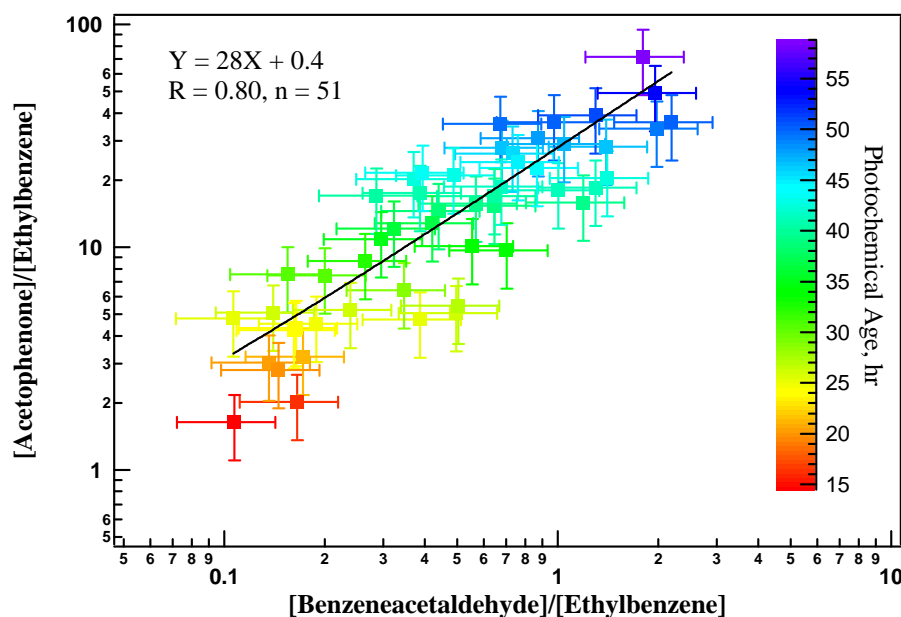
Fig. 6. Correlation between the ratios [acetophenone]/[ethylbenzene] and [benzeneacetaldehyde]/[ethylbenzene]. The vertical and horizontal bars represent the estimated errors in the ratios. Photochemical ages, as derived from the [acetophenone]/[ethylbenzene] ratios, are coded in color.
