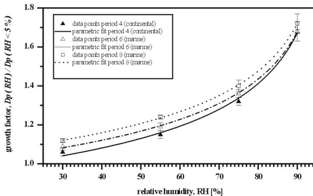
Fig. 9. Parametric fit of hygroscopic growth factors (more-hygroscopic particle fraction) measured at 30, 55, 75 and 90% RH for particles with dry particle diameter D_p = 50 nm measured for different air masses during Aerosols99. The error bars display the standard deviation of the averaged measured values.
