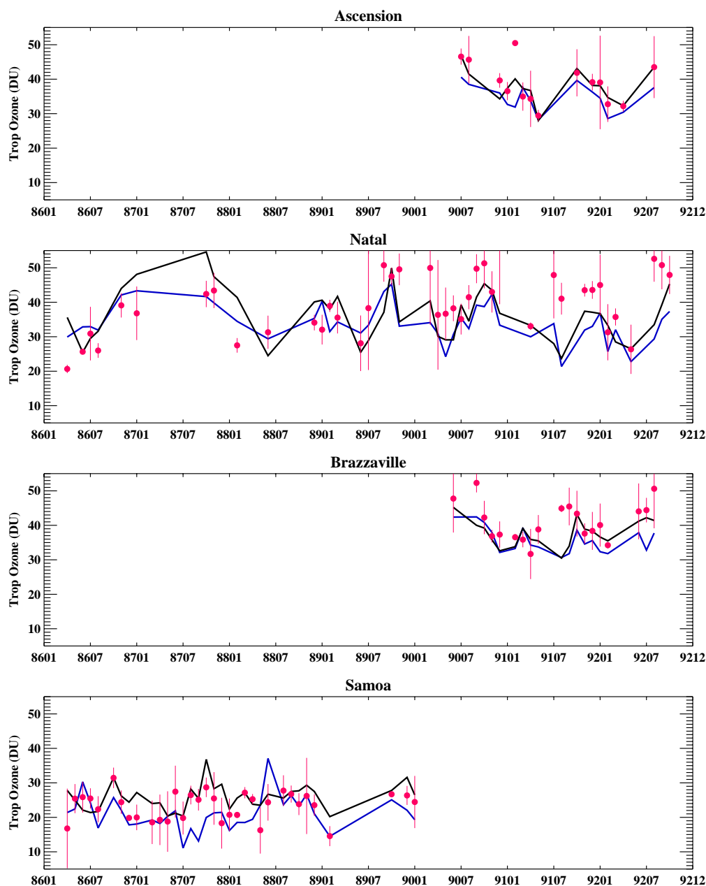
Fig. 7. Comparison of Nimbus-7 CCD and CCP tropospheric ozone with sonde measurements at four stations – Ascension Island, Natal, Brazzaville, and Samoa – over 1986–1992. Red circles are the sonde integrated tropospheric ozone columns, vertical bars represent 1 SD of the ozonesonde monthly mean, black lines represent the CCD tropospheric columns, and blue lines represent the derived CCP tropospheric columns.
