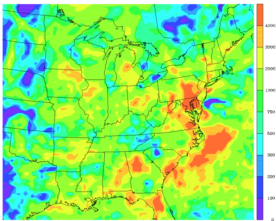
Fig. 3. Calculated total wet deposition of \text{Hg}^0 ( \text{ng m}^{-2} ) over the period of 20 June 1995 to 18 July 1995.
