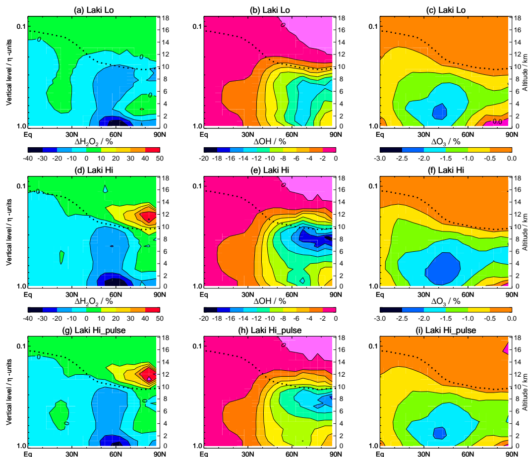
Fig. 4. Northern Hemisphere zonal, June-July-August (JJA) mean oxidant depletions (%) for Laki Lo (a–c), Laki Hi (d–f), and Laki Hi-pulse (g–i), relative to 1860. For each case, changes are plotted for: \text{H}_2\text{O}_2 (a, d, g); OH (b, e, h); and \text{O}_3 (c, f, i). The dotted line is the tropopause.
