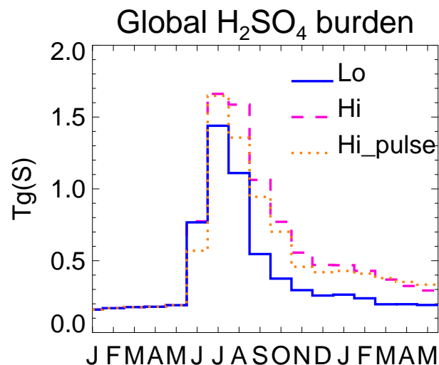
Fig. 11. Monthly global H 2 SO 4 burden (Tg(H 2 SO 4 )), for the three Laki scenarios.
