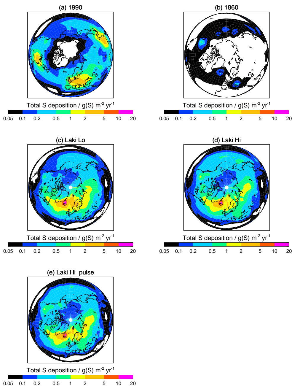
Fig. 9. Northern Hemisphere annual mean total sulphur deposition fluxes ( \text{g(S)} \text{ m}^{-2} \text{ yr}^{-1} ) for: (a) 1990; (b) 1860; (c) Laki Lo; (d) Laki Hi; and (e) Laki Hi_pulse.
