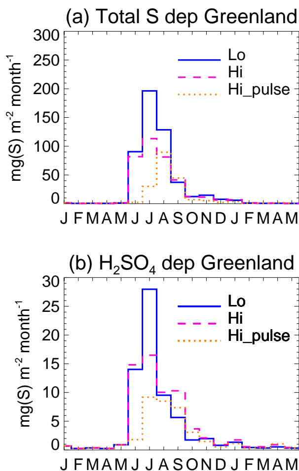
Fig. 10. Simulated monthly (a) total sulphur and (b) H 2 SO 4 deposition fluxes (mg(S) m -2 month -1 ) to central Greenland, for the three Laki scenarios.
