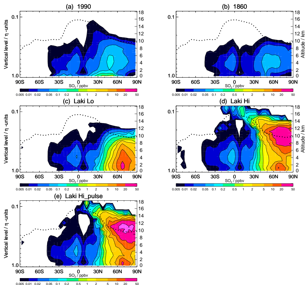
Fig. 2. Zonal, June-July-August (JJA) mean \text{SO}_2 concentrations (ppbv) for: (a) 1990; (b) 1860; (c) Laki Lo; (d) Laki Hi; and (e) Laki Hi_pulse. The dotted line is the tropopause.
