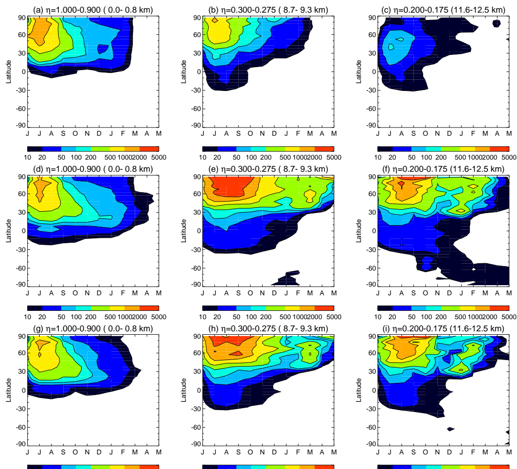
Fig. 8. Temporal evolution of the zonal mean Laki SO 4 (pptv) for Laki Lo (a–c), Laki Hi (d–f) and Laki Hi_pulse (g–i) at three levels in the model: the surface (a, d, g); the upper troposphere (b, e, h); and the lower stratosphere (c, f, i). Background 1860 levels have been subtracted.
