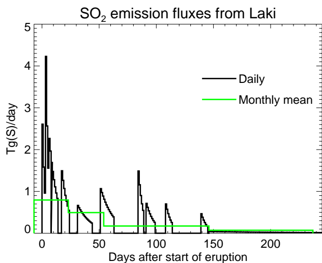
Fig. 1. Laki \text{SO}_2 emissions. Monthly mean emissions are derived from Thordarson et al. (1996) and are used in the Laki Lo and Hi scenarios. Daily emissions are derived from Thordarson and Self (2003), and assume emissions fall to (1/e) of their initial value by the final day of each episode. Daily emissions are used in the Hi_pulse scenario. Note that monthly emissions differ somewhat between the two cases, but total emissions are the same.
