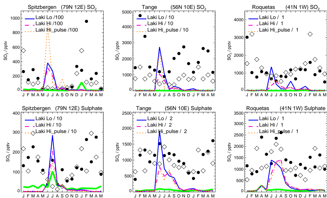
Fig. 7. Comparison of 1990 modelled surface \text{SO}_2 and \text{SO}_4 (●) with recent observations (◇) (Hjellbrekke et al., 1996) at 3 European sites. The plot extends over 17 months of model results; observations are repeated for the second year. Also shown are results from the 1860 scenario (thick green line), and the three Laki scenarios (solid blue, dashed magenta and dotted brown lines), reduced by up to a factor of 100 to fit on the plots.
