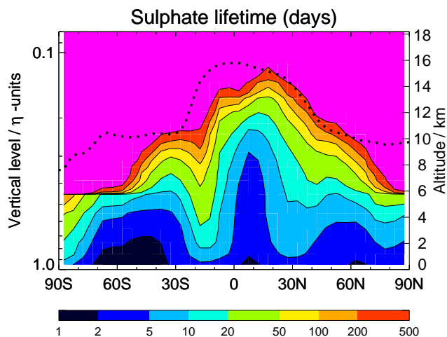
Fig. 6. Zonal, June-July-August (JJA) mean \text{SO}_4 lifetime (days) for the five scenarios (all scenarios are the same). The dotted line is the tropopause.
