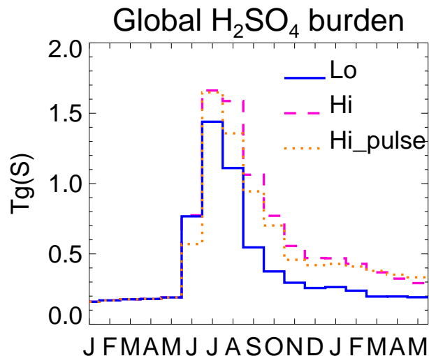
Fig. 11. Monthly global \text{H}_2\text{SO}_4 burden ( \text{Tg}(\text{H}_2\text{SO}_4) ), for the three Laki scenarios.
