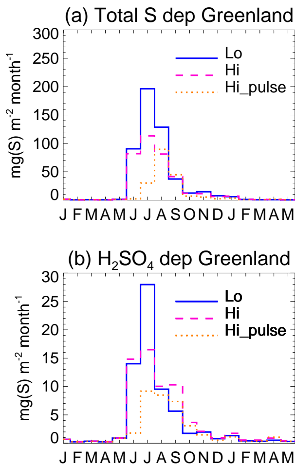
Fig. 10. Simulated monthly (a) total sulphur and (b) \text{H}_2\text{SO}_4 deposition fluxes ( \text{mg}(\text{S}) \text{m}^{-2} \text{month}^{-1} ) to central Greenland, for the three Laki scenarios.
