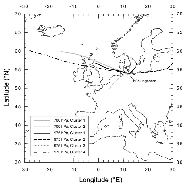
Fig. 10. Map of central Europe, showing the results of the cluster analysis of the backward trajectories arriving above Kühlungsborn ( 54^\circ N, 12^\circ E) at 19:00 UT on the measurement days. Two arrival heights are shown. Gray lines: 700 hPa, black lines: 975 hPa.
