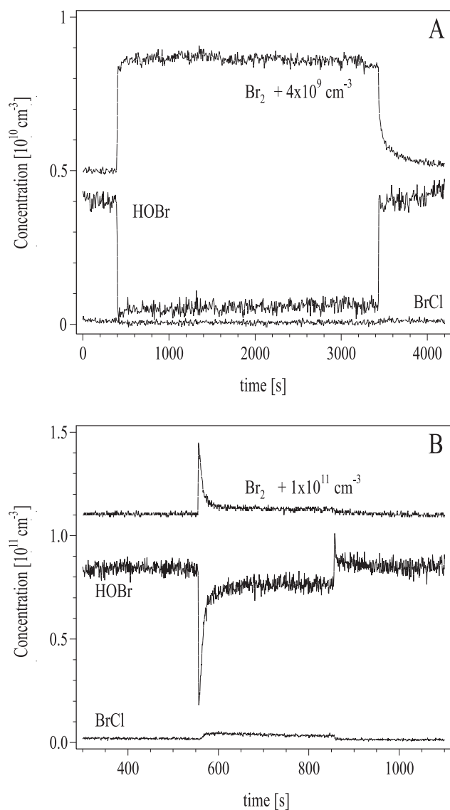
Fig. 3. Uptake of HOBr and subsequent product formation, on a frozen mixed salt surface at 233 K. (a) [\text{HOBr}]_{\text{init}} = 4 \times 10^9 \text{ molecules cm}^{-3} , exposure of the surface to HOBr begins at 400 s when the injector is retracted. (b) [\text{HOBr}]_{\text{init}} = 8.5 \times 10^{10} \text{ molecules cm}^{-3} , exposure of the surface to HOBr begins at 550 s. In both cases, the Br 2 trace has been offset for clarity of presentation.
