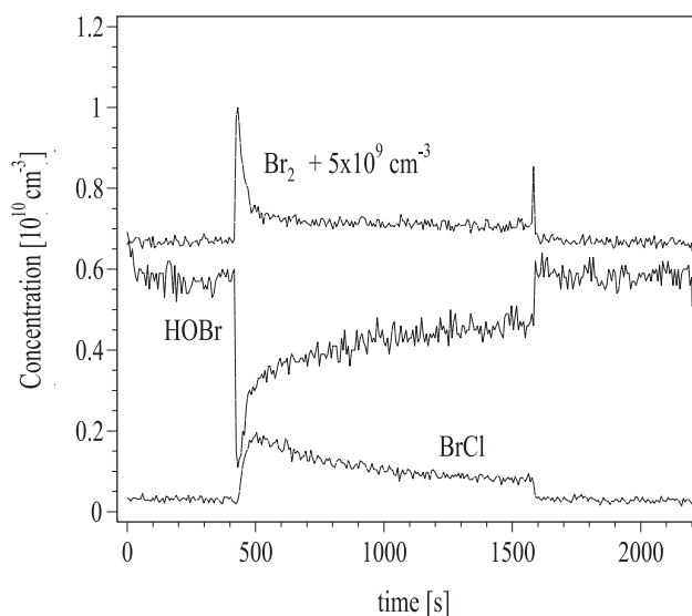
Fig. 4. Uptake of HOBr onto a frozen (233 K) mixed salt surfaces made from an aqueous solution of composition 2 M NaCl, 3 \times 10^{-4} M NaBr. The Br 2 trace has been offset for clarity of presentation.
