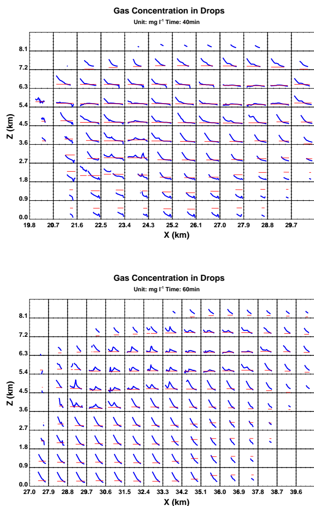
Fig. 11. As Fig. 10 but for H^* = 10^6 \text{ mol dm}^{-3} \text{ atm}^{-1} .
