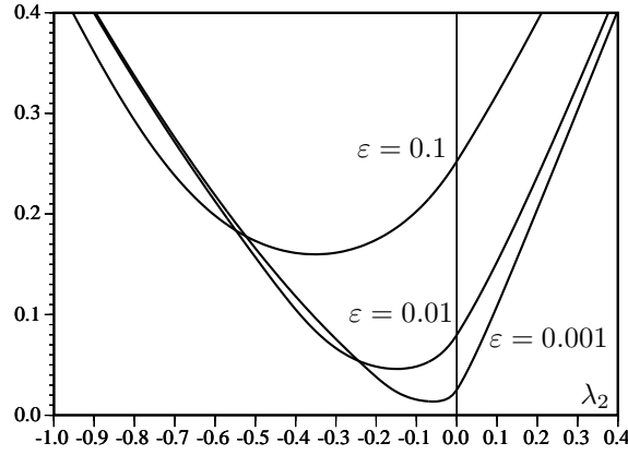
FIGURE 10. \lambda_2 -dependence of the prefactor of the expected transition time for the model system (4.1) for N = 3 .
