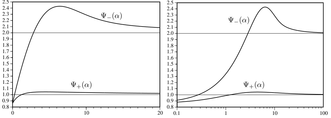
FIGURE 5. The functions \Psi_{\pm}(\alpha) , shown on a linear and on a logarithmic scale.
