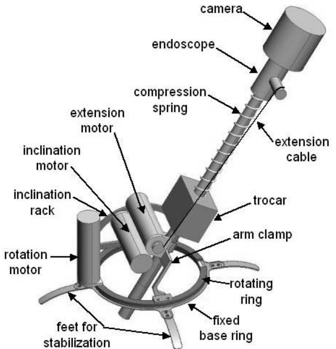
Fig. 1. Light Endoscope Robot
