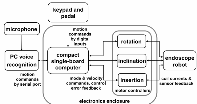
Fig. 2. Control system schematic
