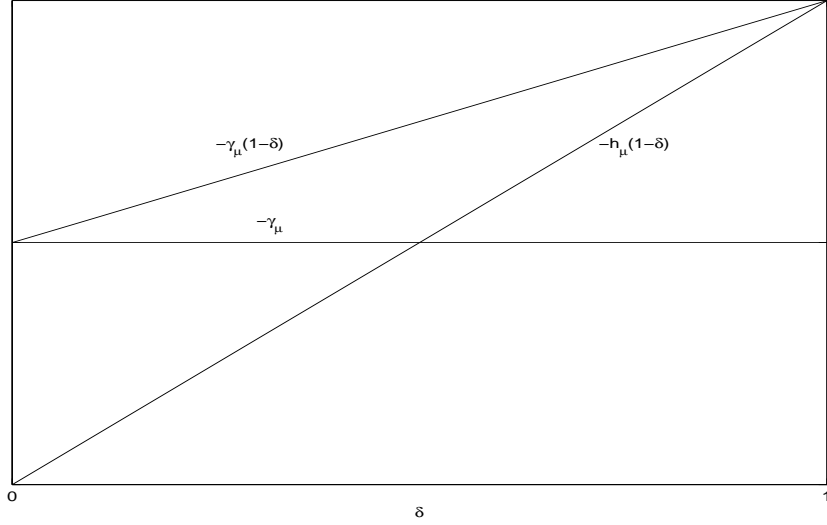
FIGURE 1. Propositions 1 and 3
