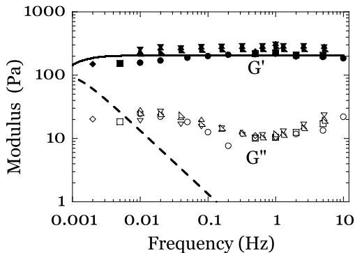
FIG. 4: Frequency dependence of G' (closed symbols) and G'' (open symbols) measured for three different samples. The shear strain amplitude is equal to 0.01. The solid and dotted lines represent the elastic and loss moduli predicted by the Maxwell model (Eq. 1) with G_0 = 206 Pa and \tau = 246 s.
