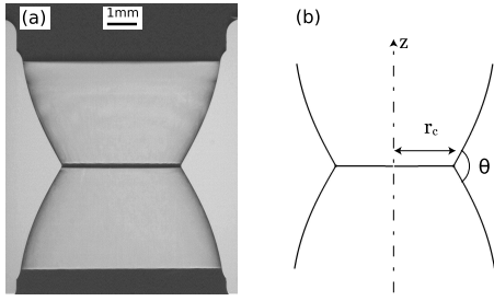
FIG. 1: (a) Two bubbles in contact, observed during an adhesion experiment. (b) Adhesion profile obtained after image analysis. The shape of the bubbles is fitted using the Young-Laplace equation and the contact radius r_c and the contact angle \theta are determined from the intersection of the reconstructed profiles.
