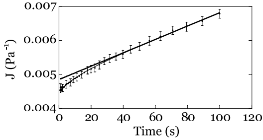
FIG. 3: Time evolution of the compliance J(t) = \varepsilon(t)/\sigma_0 during a creep experiment with a constant applied stress \sigma_0 applied during 100 s. The compliance is averaged over 4 different samples and 3 values of applied stresses comprised between 3 Pa and 6 Pa. The dotted line corresponds to the prediction of the Maxwell model Eq. (3), fitted to the data for t > 28 s. times larger than 28 s.
