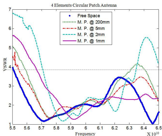
Figure 1. Measured results on the influence of a Metal Plane (M.P.) on Antenna VSWR.
