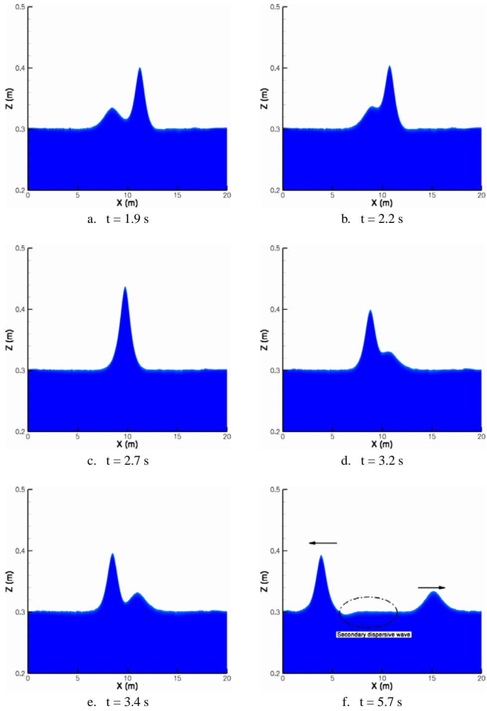
FIG. 2 – Details of the first collision at various instants. C > 0.5 .
