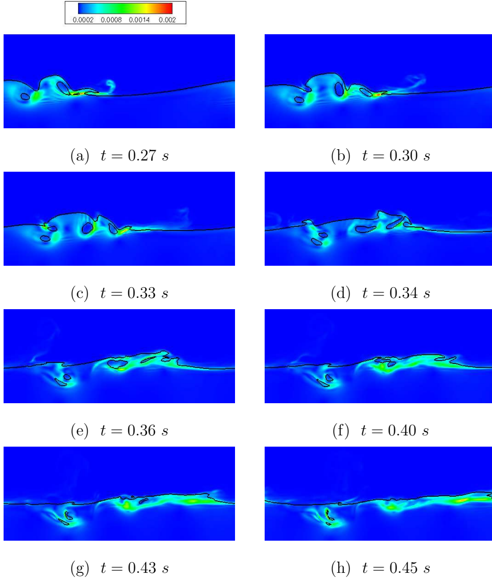
Fig. 22. Turbulent viscosity magnitude ( m^2.s^{-1} ) in both air and water media. The black line stands for C = 0.5 . Sections taken in the middle plane of a 3D simulation. \frac{H}{L} = 0.13 , \frac{d}{L} = 0.17 .
