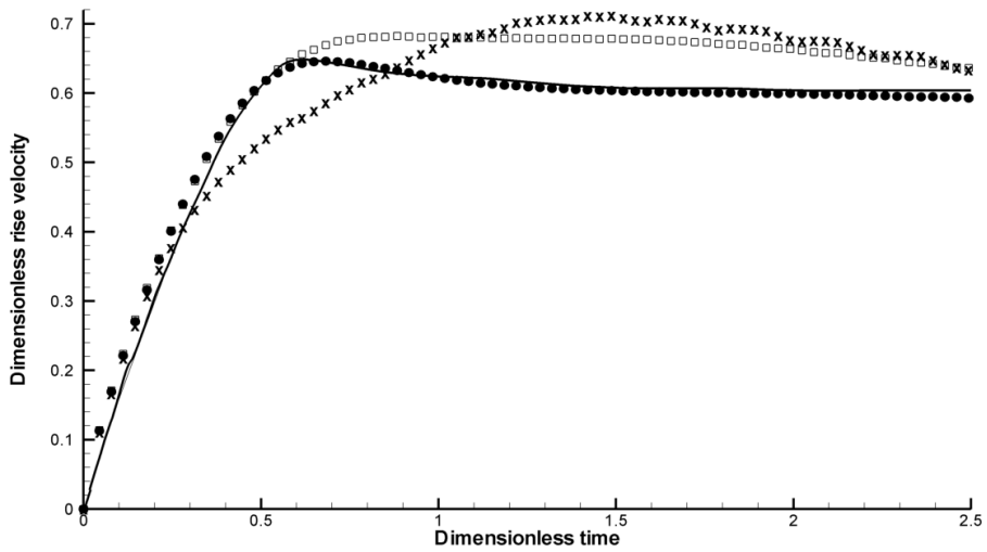
Fig. 2. Comparison between Direct Numerical Simulation (solid line) from Blanco-Alvarez (1995) and our numerical results: \bullet fine grid 69 \times 69 \times 115 , \square intermediate grid 35 \times 35 \times 56 , \times coarse grid 18 \times 18 \times 99 .
