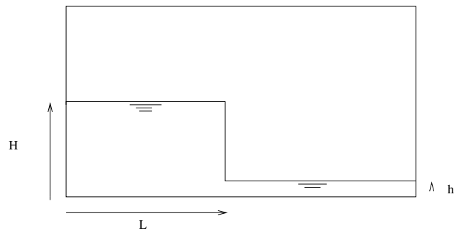
Fig. 4. Sketch of the initial condition for the dam-break problem.
