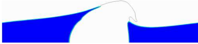
Fig. 10. Impacting jet. Sections taken from a 3D simulation. \frac{H}{L} = 0.13 , \frac{d}{L} = 0.13 , C = 0.5 .
