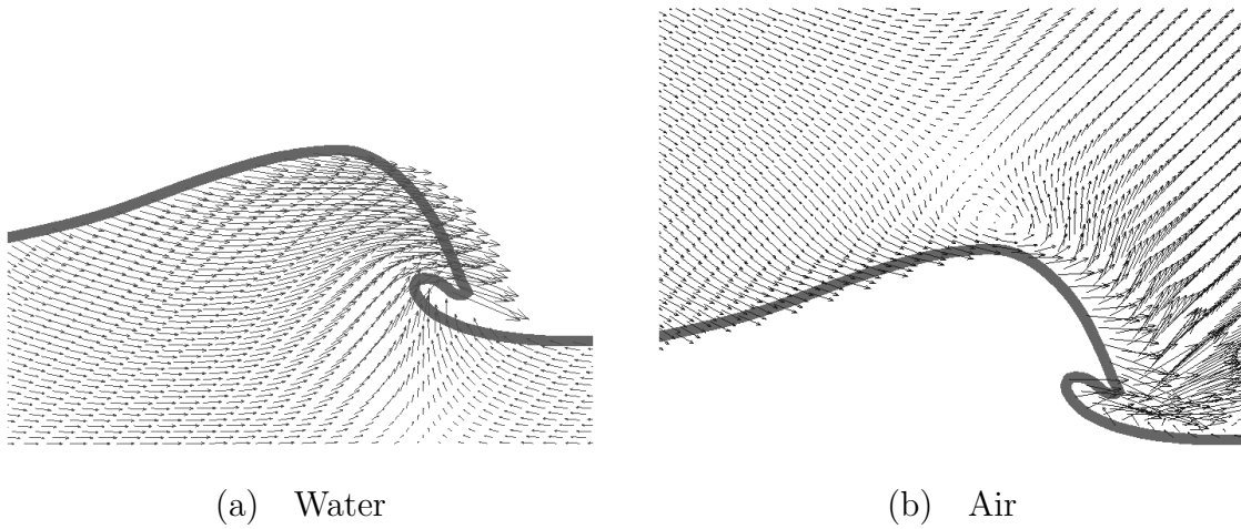
Fig. 9. Velocity field in both media. Only one vector over three is shown in each medium. Sections taken from a 3D simulation. t = 0.39 T s , C = 0.5 .
