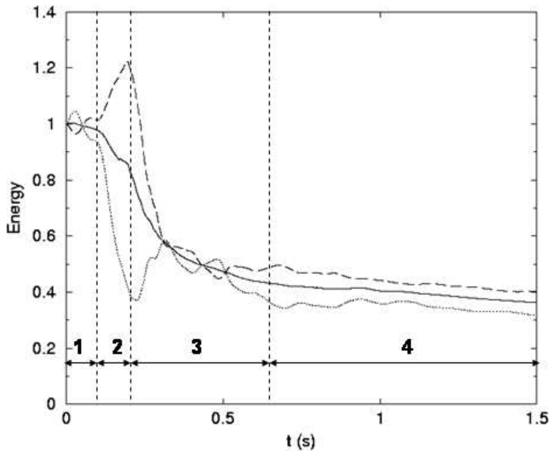
Fig. 23. Time evolution of the non-dimensional energies. Solid line: total energy; dashed line: kinetic energy; dotted line: potential energy. \frac{H}{L} = 0.10 , \frac{d}{L} = 0.10 . Zone 1: steepening of the wave; zone 2: jet ejection; zone 3: jet impact and splash-ups generation; zone 4: residual flow.
