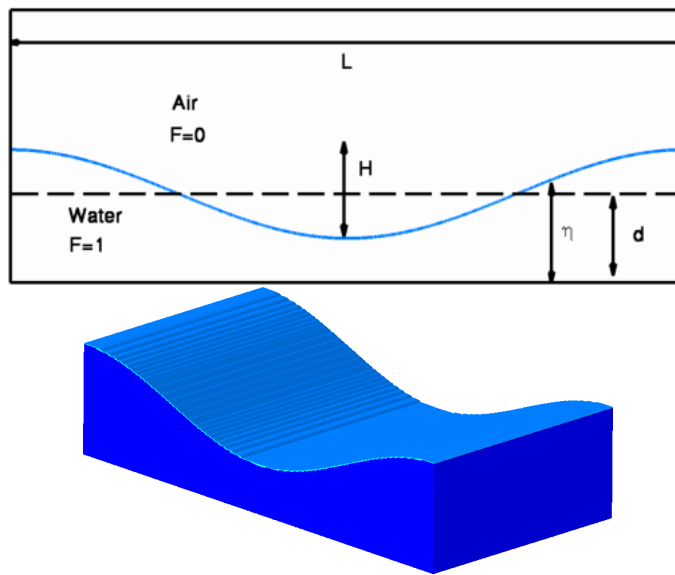
Fig. 7. Sketch of the initial condition for the unstable periodic sinusoidal wave of large amplitude (2D/3D). \frac{H}{L} = 0.13 , \frac{d}{L} = 0.17 , t = 0 s, C \geq 0.5 .
