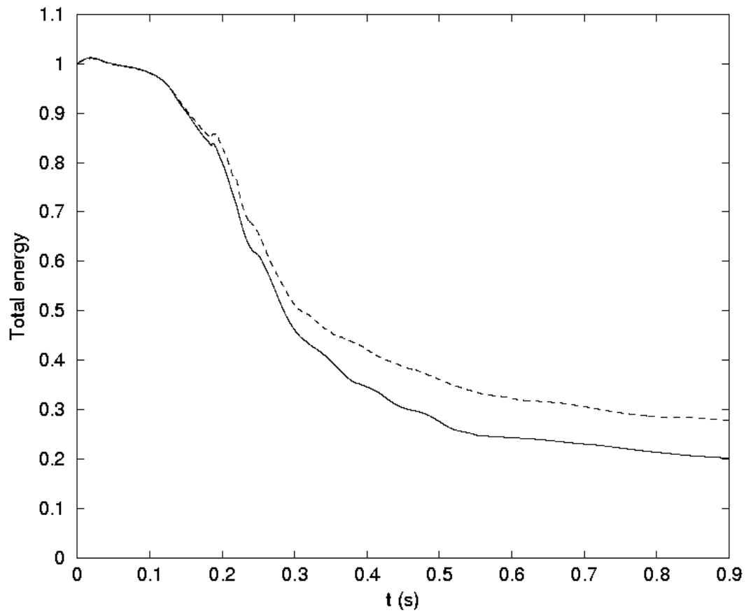
Fig. 24. Time evolution of the non-dimensional energy. Solid line: total energy calculated from a 3D simulation; dashed line: total energy calculated from a 2D simulation. \frac{H}{L} = 0.10 , \frac{d}{L} = 0.10 .
