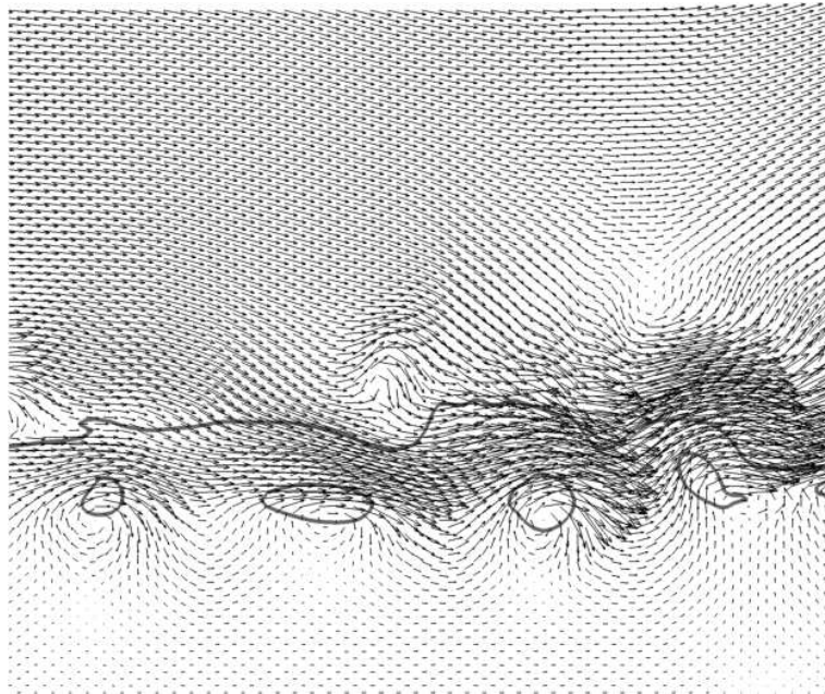
Fig. 15. Co-rotative vortices. Only one vector over two is shown in the water. \frac{H}{L} = 0.08 , \frac{d}{L} = 0.10 , C > 0.5 .
