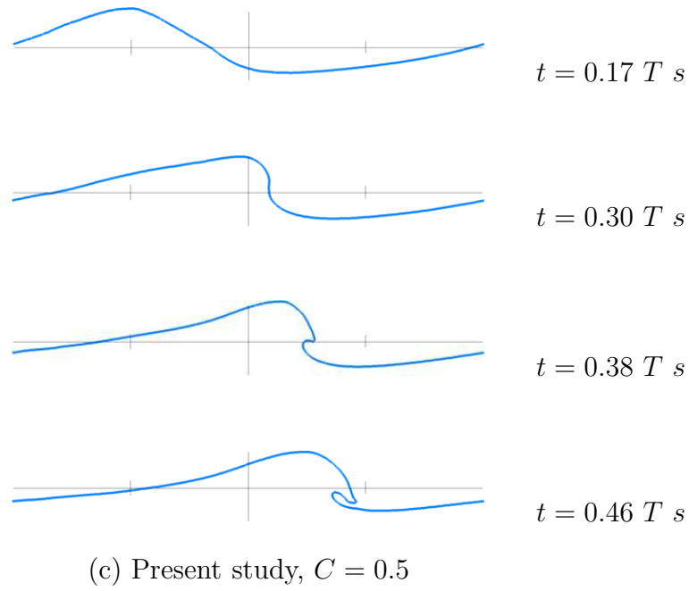
Fig. 8. Time evolution of the overturning motion. Sections taken from a 3D simulation. \frac{H}{L} = 0.13 , \frac{d}{L} = 0.13 .
