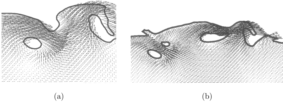
Fig. 14. Splash-up generation. Sections taken from a 3D simulation. Only one vector over three is shown in the water. \frac{H}{L} = 0.13 , \frac{d}{L} = 0.13 , C = 0.5 .
