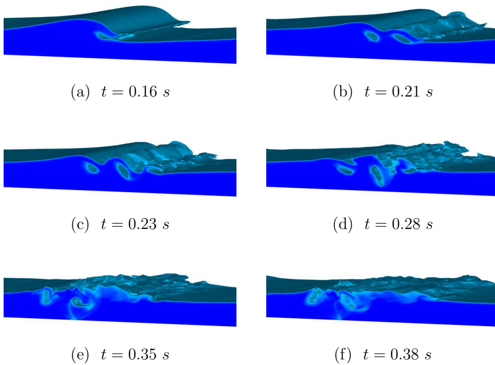
Fig. 20. Snap shots of a three-dimensional large eddy simulation of a plunging breaker. \frac{H}{L} = 0.10 , \frac{d}{L} = 0.10 , C \geq 0.5 .
