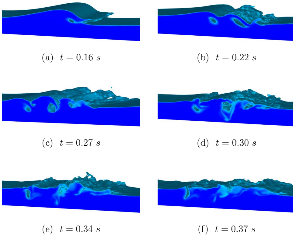
Fig. 19. Snap shots of a three-dimensional large eddy simulation of a plunging breaker. \frac{H}{L} = 0.13 , \frac{d}{L} = 0.13 , C \geq 0.5 .
