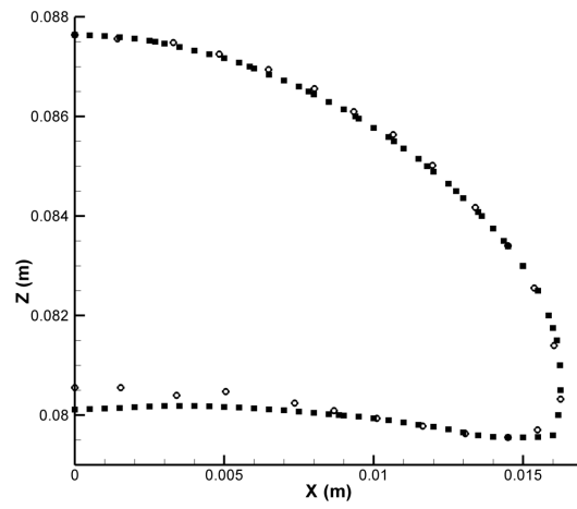
Fig. 3. Comparison between experimental free surface profiles ( \circ ) from Hnat and Buckmaster (1976) and three-dimensional numerical results ( \blacksquare ) for the final shape of a rising bubble.
