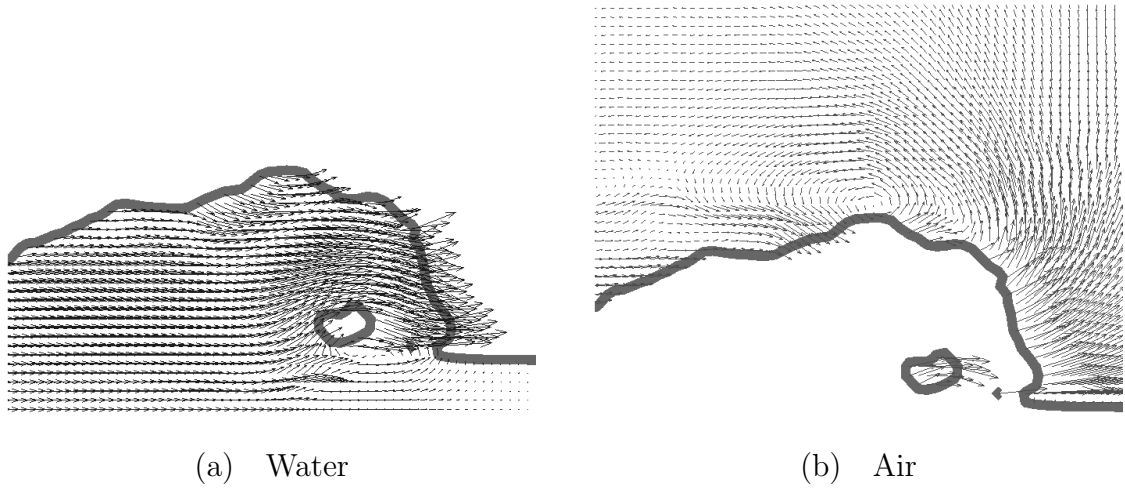
Fig. 6. Velocity field in both media. t = 0.24 s, C = 0.5 .
