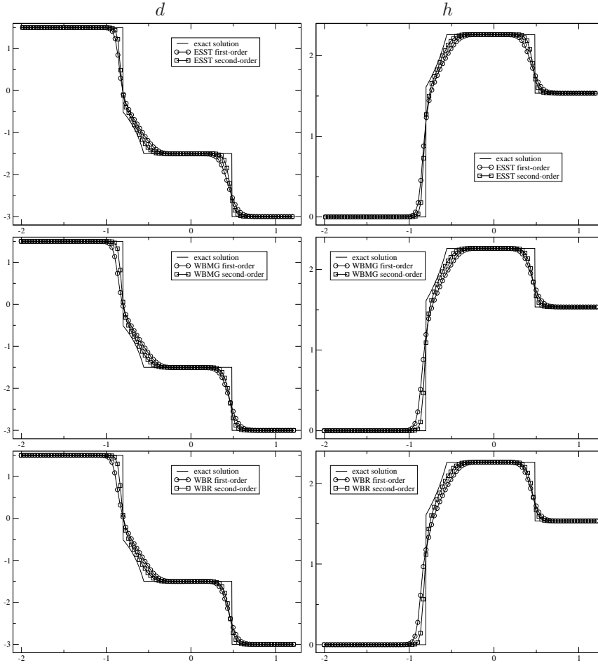
FIGURE 4. Riemann problem 1: d and h with first and second order schemes ESST, WBR and WBMG on the interval (-2.0039, 1.2113) with a uniform mesh made of 100 cells
