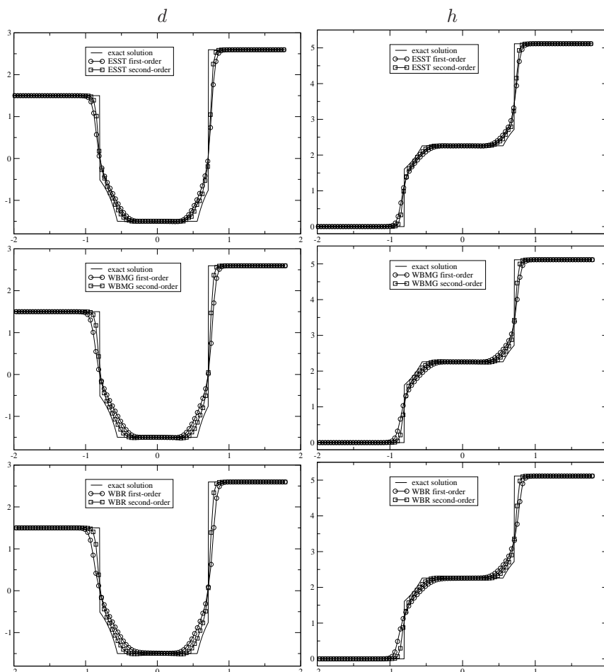
FIGURE 6. Riemann problem 2: d and h with first and second order schemes ESST, WBR and WBMG on the interval (-2.0039, 1.7831) with a uniform mesh made of 100 cells
