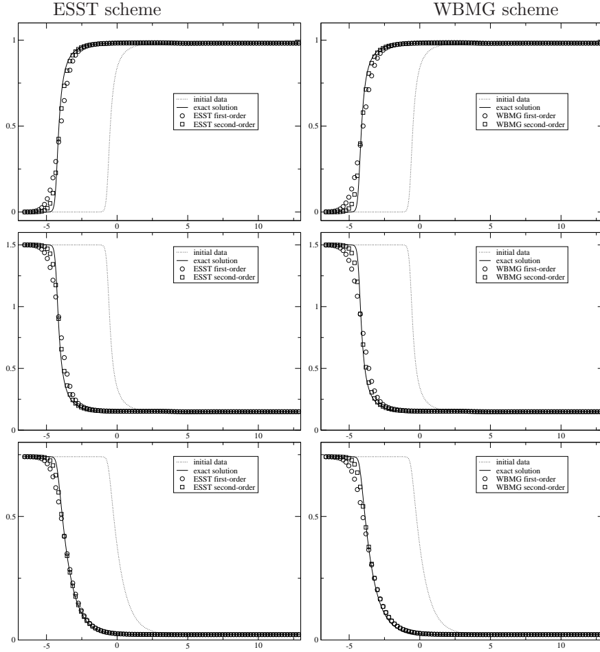
FIGURE 3. Relaxation shock profile 2: d , h and \chi with first and second order schemes ESST and WBMG with a uniform mesh made of 100 cells
