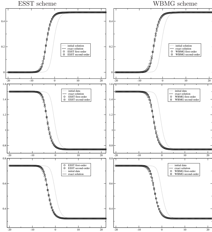
FIGURE 2. Relaxation shock profile 1: d , h and \chi with first and second order schemes ESST and WBMG with a uniform mesh made of 100 cells
