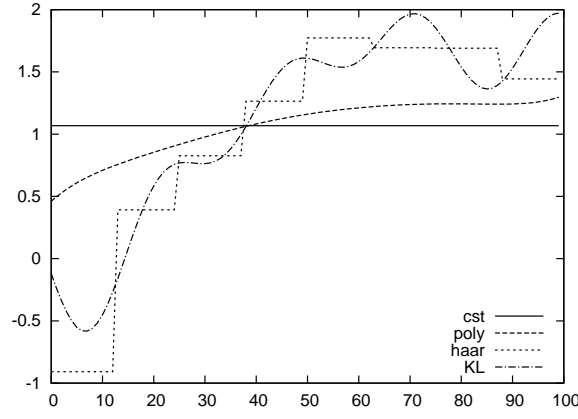
(c) 8 vectors
