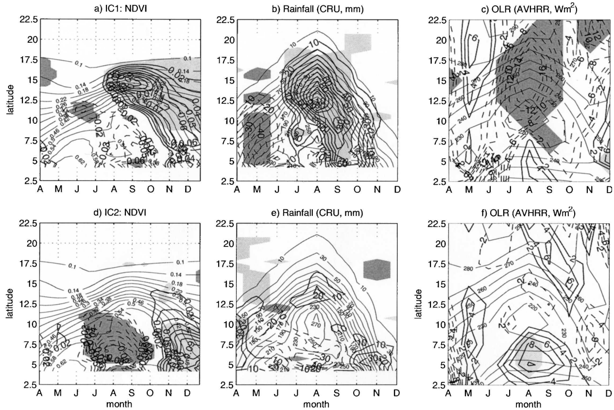
FIG. 3. Time–latitude diagrams (from 2.5° to 22.5°N and April to December) of composite differences of NDVI (unitless), rainfall (from CRU dataset, mm), and OLR ( \text{W m}^{-2} ) averaged over 18°W–18°E with respect to years of high minus low NDVI for (a)–(c) IC1 and (d)–(f) IC2. Solid red (dashed blue) lines enclose positive (negative) differences. Shading indicates differences significant at the 95% level according to a Student's t test. Black solid lines display the mean annual cycle.
