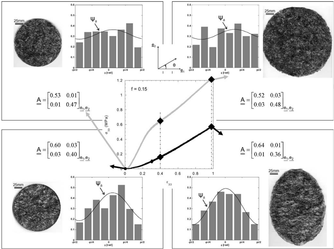
Fig. 7 Example of two simple compression tests performed on two specimens ( f = 0.15 ) with initial random ( A_{11}^{\text{init}} \approx 0.5 ) and oriented ( A_{11}^{\text{init}} \approx 0.6 ) microstructures. The centered graph gives the recorded axial Cauchy stresses \sigma_{33} and logarithmic strains \epsilon_{33} .
