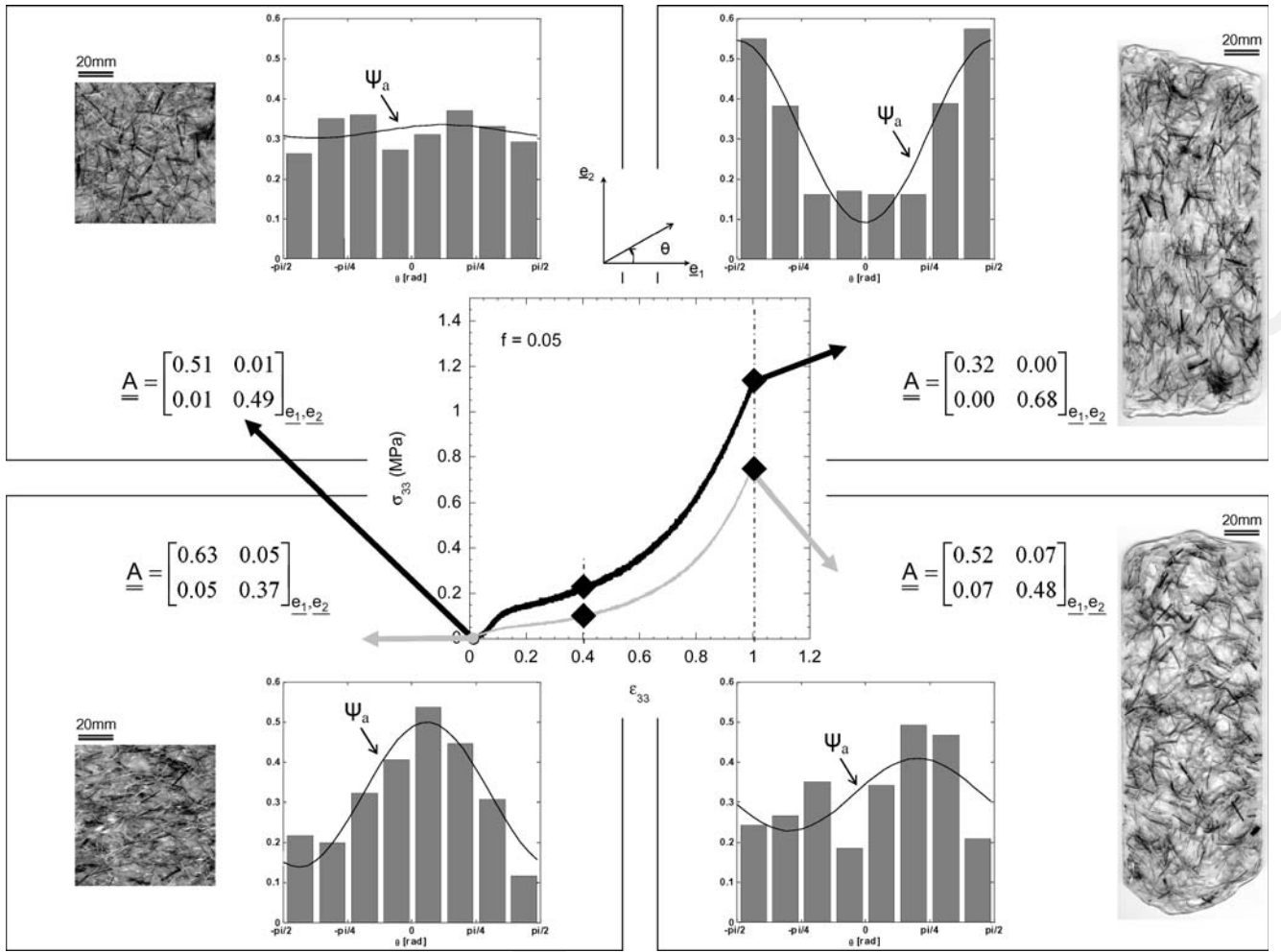
Fig. 8 Example of two plane strain compression tests performed on two specimens ( f = 0.05 ) with initial random ( A_{11}^{\text{init}} \approx 0.5 ) and oriented ( A_{11}^{\text{init}} \approx 0.6 ) microstructures. The centered graph gives the recorded axial Cauchy stresses \sigma_{33} and logarithmic
