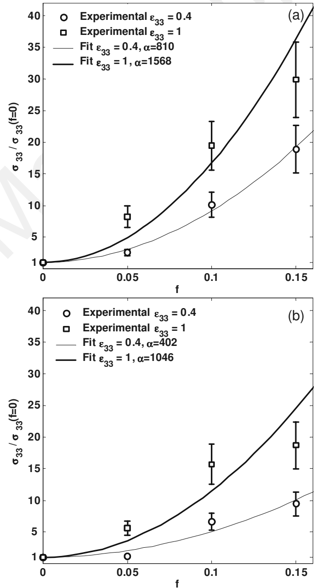
Fig. 10 Plane strain compressions—influence of the volume fraction of fibres f on stress ratios \sigma_{33}(f)/\sigma_{33}(f=0) measured at two axial logarithmic strains, i.e. \varepsilon_{33} = 0.4 and \varepsilon_{33} = 1 . Initially random (a) and oriented (b) microstructures
