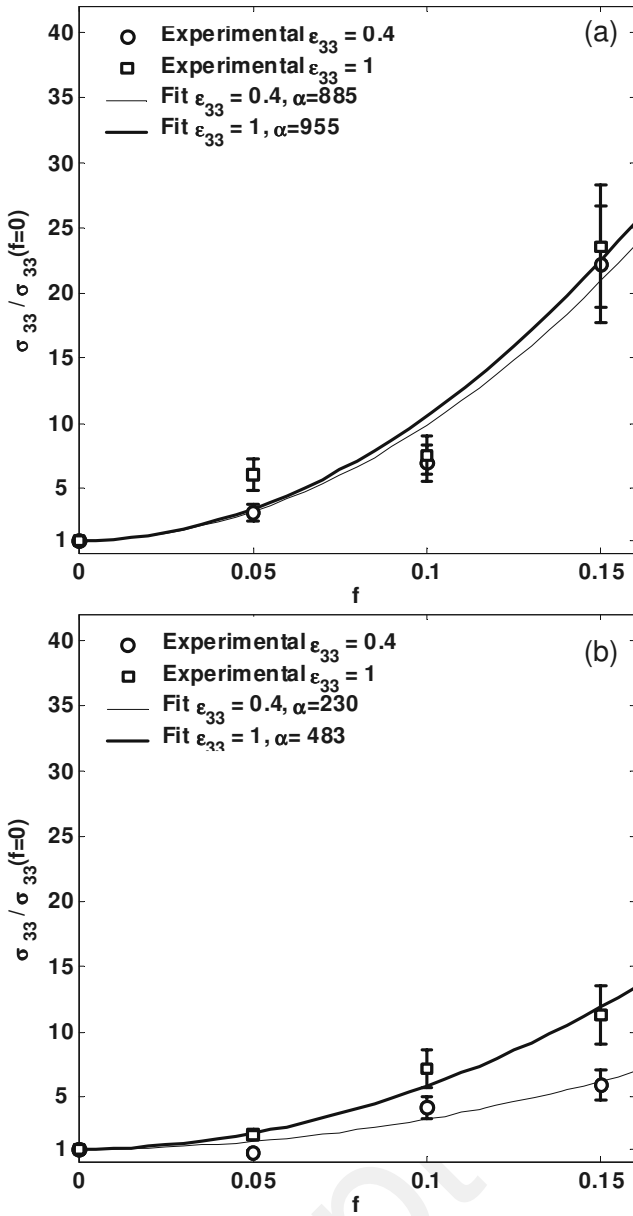
Fig. 9 Simple compressions—influence of the volume fraction of fibres f on stress ratios \sigma_{33}(f)/\sigma_{33}(f=0) measured at two axial logarithmic strains, i.e. \varepsilon_{33} = 0.4 and \varepsilon_{33} = 1 . Initially random (a) and oriented (b) microstructures
