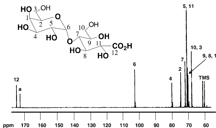
Fig. 6. NMR- 13 C spectrum of the reaction product obtained at the end of electrolysis of 10.1 mM lactose on gold nanoparticle modified carbon felt electrode in carbonate buffer (pH 10.2) at 1.2 V(RHE).
