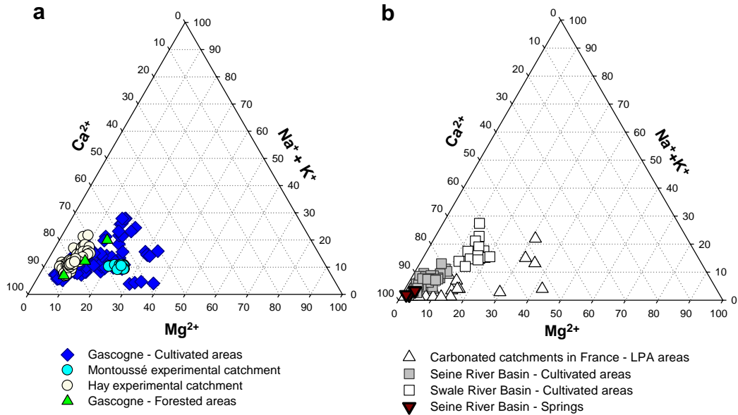
Fig. 3. Cation ternary diagram: (a) stream water samples from cultivated and forested areas of the Gascogne region and from the Montoussé and Hay experimental catchments; (b) stream water samples from carbonate areas with low anthropogenic pressure (LAP) in France (Meybeck, 1986), from cultivated areas and spring areas of the Seine basin (Roy et al., 1999), and from cultivated areas in the Swale basin (House and Warwick, 1998) compared to Gascogne cultivated catchments.
