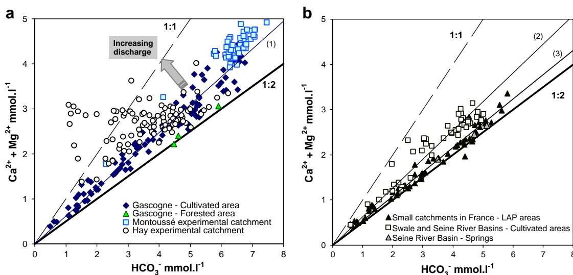
Fig. 6. Relationship between ( \text{Ca}^{2+} + \text{Mg}^{2+} ) and \text{HCO}_3^- concentrations in stream waters: (a) samples from cultivated and forested areas of the Gascogne and from the Montoussé and Hay experimental catchments; (b) samples from small carbonate catchments with low anthropogenic pressure (LAP) in France (Meybeck, 1986), from the cultivated and spring areas of the Seine river basin (Roy et al., 1999) and from the cultivated areas of the Swale river basin (House and Warwick, 1998). Regression equations are as follows: (1) cultivated catchments of the Gascogne y = 0.6x , r^2 = 0.95 ( p \leq 0.001 ), n = 80 ; (2) cultivated catchments of the Swale river and Seine river basins: y = 0.7x , r^2 = 0.89 ( p \leq 0.001 ), n = 47 ; (3) French streams with low anthropogenic pressure: y = 0.5x , r^2 = 0.97 , n = 57 ( p \leq 0.001 ). Theoretical line 1:2 (corresponding to expected \text{Ca}^{2+} + \text{Mg}^{2+}/\text{HCO}_3^- ratio according to Eq. 2) is indicated.
