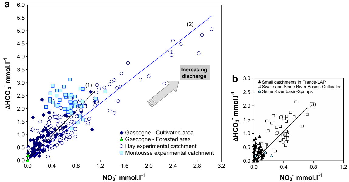
Fig. 7. Relationship between \Delta\text{HCO}_3^- ( \text{HCO}_3^-_{\text{theoretical}} - \text{HCO}_3^-_{\text{measured}} ; \text{mmol l}^{-1} ) and \text{NO}_3^- concentrations ( \text{mmol l}^{-1} ) in surface waters: (a) samples from cultivated and forested areas of the Gascogne and from the Montoussé and Hay experimental catchments; (b) samples from French catchments with low anthropogenic pressure (Meybeck, 1986), from the cultivated and spring areas of the Seine river basin (Roy et al., 1999) and from the cultivated areas of the Swale river basin (House and Warwick, 1998). Regression equations are as follows: (1) cultivated catchments of the Gascogne y = 2.4x , r^2 = 0.43 ( p \leq 0.001 ), n = 80 ; (2) Hay experimental catchment y = 1.8x , r^2 = 0.76 ( p \leq 0.001 ), n = 100 ; (3) cultivated catchments of the Swale and Seine basins: y = 2.7x , r^2 = 0.21 ( p \leq 0.001 ), n = 47 .
