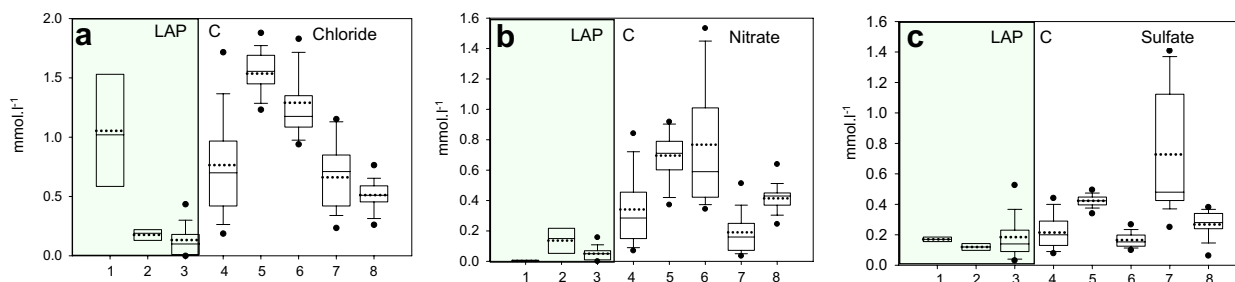
Fig. 5. Box Plot representing statistical values for chloride (a), nitrate (b) and sulfate (c). (LAP) means Low Anthropogenic Pressure areas: (1) Gascogne, n = 3 ; (2) Seine basin springs, n = 3 ; and (3) streams located in carbonate areas with LAP in France, n = 57 (Meybeck, 1986). (C) means cultivated areas: (4) Gascogne catchments, n = 80 ; (5) Montoussé experimental catchment, n = 54 ; (6) Hay experimental catchment, n = 100 ; (7) catchments located in cultivated areas in the Swale river basin, n = 15 (House and Warwick, 1998) and (8) Seine river basin, n = 32 (Roy et al., 1999). The median concentration (plain line), mean concentration (dotted line), 25th percentile (boundary of box closest to zero), 75th percentile (boundary of box farthest from zero), 90th percentile (points above the box) and 10th percentiles (points below the box) are shown.
