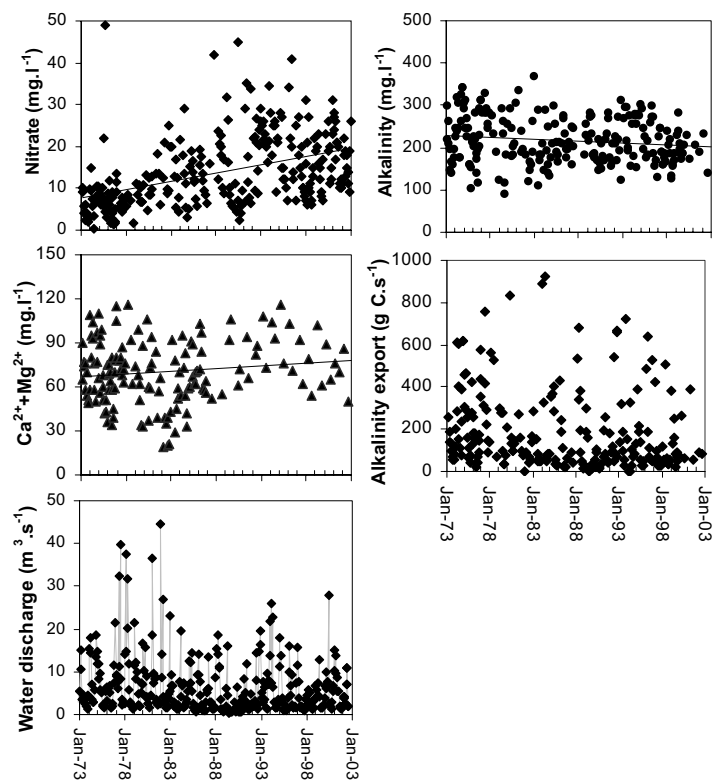
Fig. 10. Variations of bicarbonate, divalent cations ( \text{Ca}^{2+} + \text{Mg}^{2+} ), nitrate concentrations ( \text{mg l}^{-1} ), alkalinity export ( \text{g C s}^{-1} ) and discharge ( \text{m}^3 \text{s}^{-1} ) for the Save river (a main tributary of the Garonne river draining an intensively cultivated area) over the period 1973–2003. Lines represent linear regression trends over the time period (in the calculations, x is expressed in days from 01-01-1900): Alkalinity = -2.8 \cdot 10^{-3}x + 303.07 , r^2 = 0.026 , p \leq 0.05 , n = 231 ; \text{NO}_3 = 1.2 \cdot 10^{-3}x - 23.51 , r^2 = 0.21 , p \leq 0.001 , n = 275 ; \text{Ca} + \text{Mg} = 10^{-3}x + 39.64 , r^2 = 0.020 , p < 0.10 , n = 156 ; Q = -0.3 \cdot 10^{-3}x + 17.20 , r^2 = 0.033 , p \leq 0.010 , n = 364 . Data are from the French water agency Adour-Garonne.
