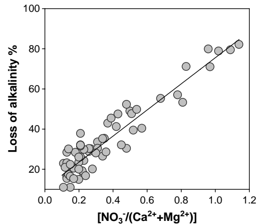
Fig. 9. Relationship between alkalinity loss (%) (expressed as [\text{HCO}_3^-_{\text{theoretical}} - \text{HCO}_3^-_{\text{measured}}]/\text{HCO}_3^-_{\text{theoretical}} ) and [\text{NO}_3^-/\text{Ca}^{2+} + \text{Mg}^{2+}] (moles. \text{l}^{-1} /moles. \text{l}^{-1} ) at the outlet of the Hay experimental catchment.
