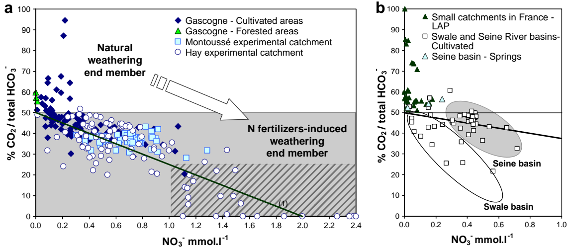
Fig. 8. Relationship between \text{CO}_2_{\text{ATM-SOIL}}/\text{total HCO}_3^- ratio (%) and \text{NO}_3^- concentrations ( \text{mmol.l}^{-1} ) in water: (a) samples from cultivated and forested areas of the Gascogne and in the Montoussé and Hay experimental catchments; (b) samples from French streams with low anthropogenic pressure (Meybeck, 1986), from the cultivated and spring areas of the Seine basin (Roy et al., 1999) and from the cultivated areas of the Swale basin (House and Warwick, 1998). (1) represents the theoretical line in the case of carbonate dissolution by protons from N-fertilizer nitrification. The equation is: \text{CO}_2_{\text{ATM-SOIL}}/\text{total HCO}_3^- = -0.25[\text{NO}_3^-] + 0.50 .
