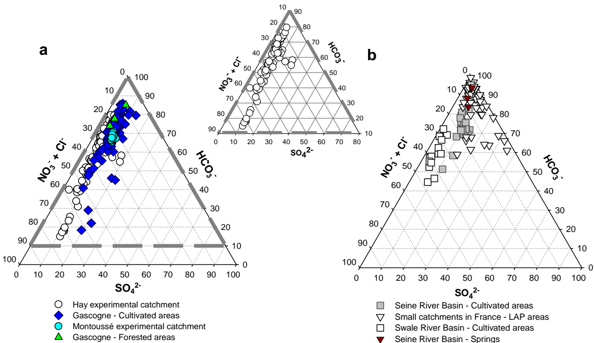
Fig. 4. Anion ternary diagram: (a) stream water samples from cultivated and forested areas of the Gascogne region and from the Montoussé and Hay experimental catchments, with a focus triangle on the Hay catchment data; (b) stream water samples from carbonate areas with low anthropogenic pressure (LAP) in France (Meybeck, 1986), from cultivated areas and spring areas of the Seine basin (Roy et al., 1999), and from cultivated areas in the Swale basin (House and Warwick, 1998), compared to Gascogne cultivated catchments.
