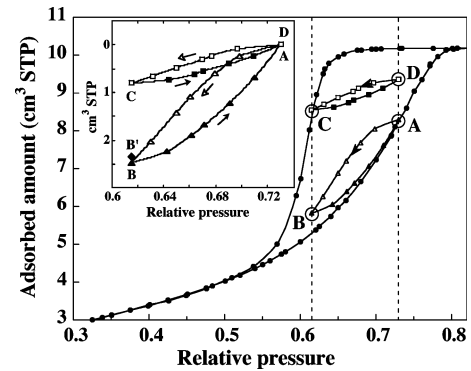
Figure 10. Hysteresis loop for sample A shown in Figure 6 with two subloops between the same pressure end points p_A and p_B , one (ABA) initiated on the primary filling branch, the other (CDC) on the primary draining branch. The inset shows the two subloops for which the right end points A and D are offset to overlap. The point B' accounts for the correction as calculated in Appendix B. This correction represents less than 8% of the observed lack of congruence which is V_{B'} - V_C = 1.66 cm 3 STP.
