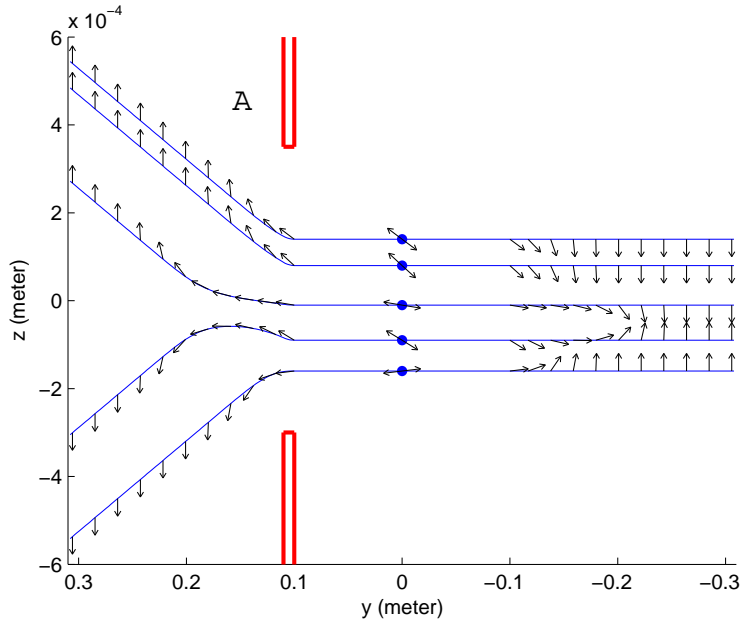
Figure 2: Five pairs of trajectories of entangled particles. Arrows represent the spin orientation.
