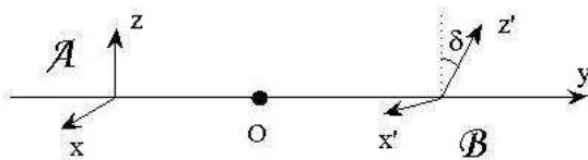
Figure 1: Schematic configuration of EPR-B experiment.
