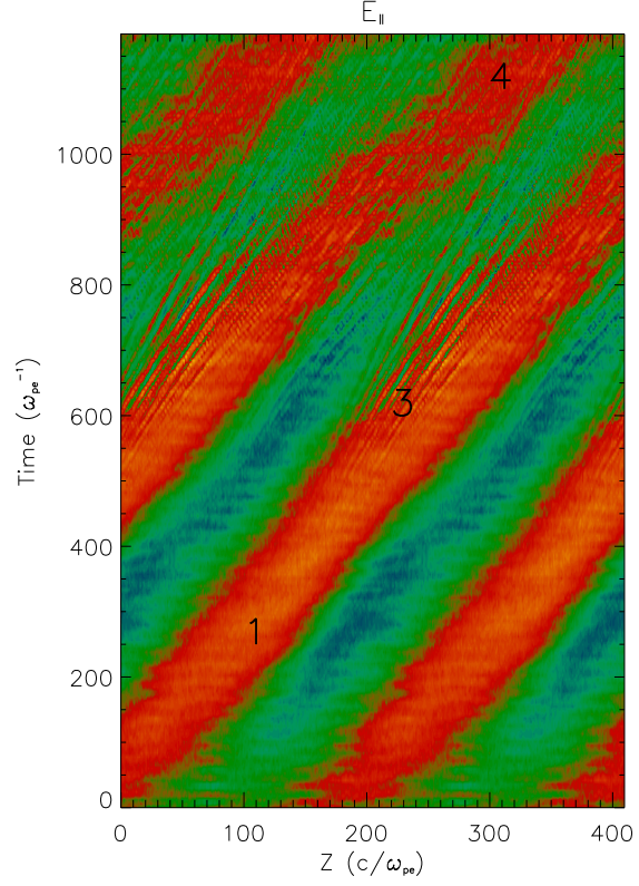
Fig. 3. Similar to Figure 2 for the low amplitude case \delta B/B = 0.025 . The Buneman instability (label 2 on Figure 2) is not triggered.
