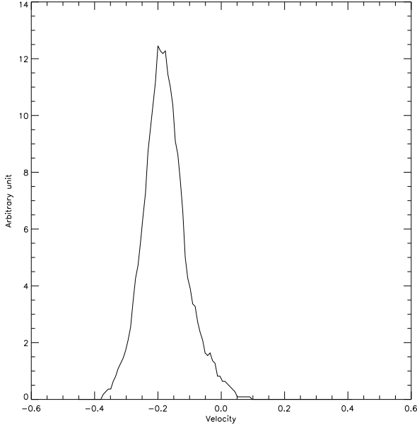
Fig. 4. Electron velocity distribution function leading to the Buneman instability at \omega_{pe}t = 320 and Z = 162c/\omega_{pe} (below label 2 on Figure 2) in the density gradient region.
