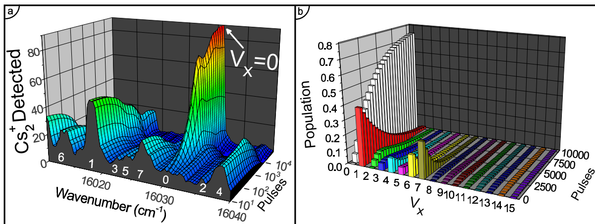
Figure 4 : Temporal evolution (pulse separation 12.5ns) of the populations in the different vibrational levels of the ground state. Due to our weak laser intensity, the excitation probability is only 0.1% for a single pulse. A , Experimental population versus the number of applied femtosecond pulses, smoothed from 5 spectra (similar to Fig.2 but taken after controlled number of pulses). The frequencies correspond to transitions from v_x = 0 - 7 to v_C levels (white label). B , Theoretical simulation where we represent the temporal evolution of v_x = 0 to 15 starting with initial conditions close to the experimental ones.
