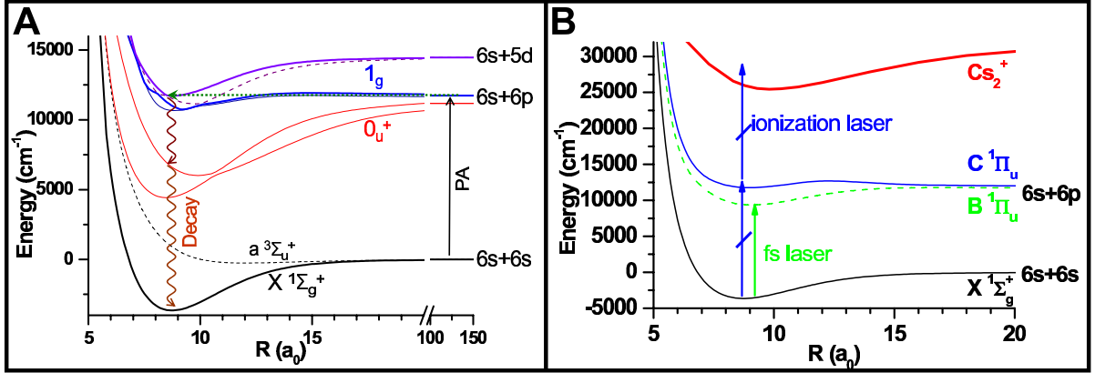
Figure 1 : Relevant schematic molecular potential curves of the cesium dimer, converging towards the dissociation limits 6s+6s , 6s+6p , and 6s+5d (for clarity, the fine structure is not labelled). A , Photoassociation of cold atoms and formation of cold molecules. The cw laser (PA) is tuned \sim 1 \text{ cm}^{-1} below the atomic transition 6s_{1/2} \rightarrow 6p_{3/2} . For the potentials of 1_g symmetry, long-range radial wavefunction is coupled to short range radial wavefunction by internal coupling of the potentials (26). The ground-state molecules, X^1\Sigma_g^+ , are formed by a spontaneous emission cascade via the 0_u^+ potentials. B , REMPI ionization process via the C^1\Pi_u state by the pulsed dye laser, and electronic transition X^1\Sigma_g^+ towards B^1\Pi_u induced by the femtosecond laser.
