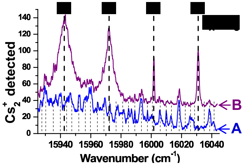
Figure 2 : Cs_2^+ ion spectra. A , Spectrum without the shaped laser pulse. The spectrum has a background due to other REMPI processes which do not mask the resonance lines. The dashed lines indicate the positions of all the resonances for vibrational transitions between the ground state, X^1\Sigma_g^+ ( v_X = 0 to 7), and the electronically excited C^1\Pi_u state ( v_C ). B , Spectrum with the shaped laser pulse applied continuously, offset by 40 ions for higher visibility. The observed transitions from v_X = 0 correspond to v_C = 0, 1, 2 and 3. Their broadening correspond to the saturation of the resonance in the REMPI process. Most of the lines present in spectrum A are greatly reduced while the v_X = 0 lines grow more intense. The resonance labeled 1-4 indicates imperfect depopulation of v_X=1 due to the roughness of the shaping.
