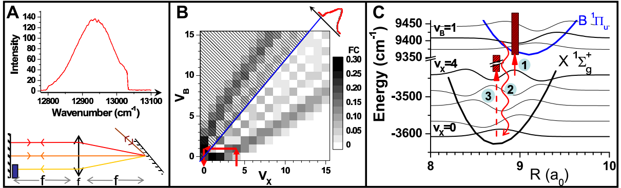
Figure 3 : Optical pumping scheme with a shaped femtosecond laser pulse. A, Upper part, the line gives the laser spectrum profile with shaping (shown also in B), close to a gaussian profile sharply cut off at 13030\text{ cm}^{-1} . Lower part, 4-f shaping arrangement (from right to left: grating; cylindrical lens f = 500\text{mm} ; blocker; mirror). B, Condon parabola indicating the importance (level of grey) of the Franck-Condon (FC) factors (square of the wavefunction overlap), corresponding to the relative transition probabilities from v_X to v_B . The diagonal line corresponds to the shaped laser cutoff frequency ( 13030\text{ cm}^{-1} ). The hatched area cannot be accessed in the presence of the blocker. C, Optical pumping scheme and vibrational wavefunctions. The vertical black boxes indicate the spectral bandwidth of the laser. In B and C, arrows indicates the optical pumping for v_X = 4 molecules. The most probable optical pumping scheme is to reach v_X = 0 through excitation into v_B = 1 . Step (1), excitation towards v_B = 1 . Step (2), spontaneous decay to v_X = 0 . Step (3), molecules in v_X = 0 are trapped. The incoherent dark state formed by the laser pulse shaping does not allow the excitation from v_X = 0 to any v_B level.
