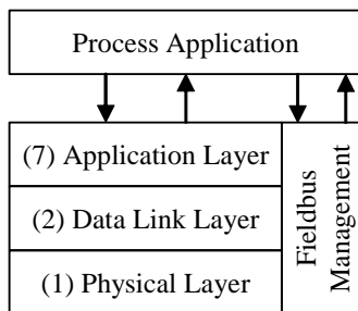
Figure 3: Fieldbus management in certain protocols
