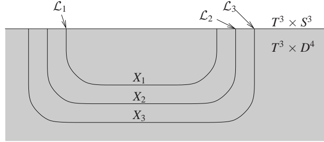
Figure 2: Submanifold X = X_1 \cup X_2 \cup X_3
