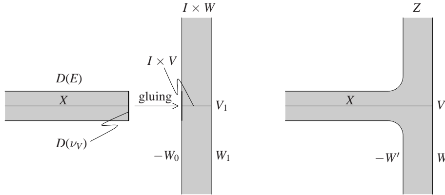
Figure 1: Gluing D(E) and I \times W , and the obtained manifold pair (Z, X)
