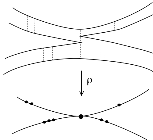
Figure 2: A regular neighborhood and the tie foliation.
