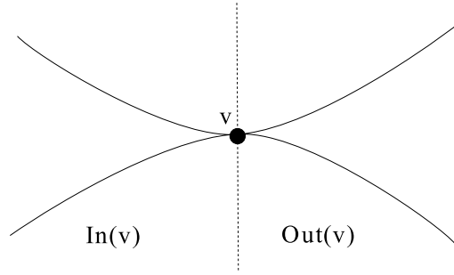
Figure 1: The smooth structure at a vertex.
