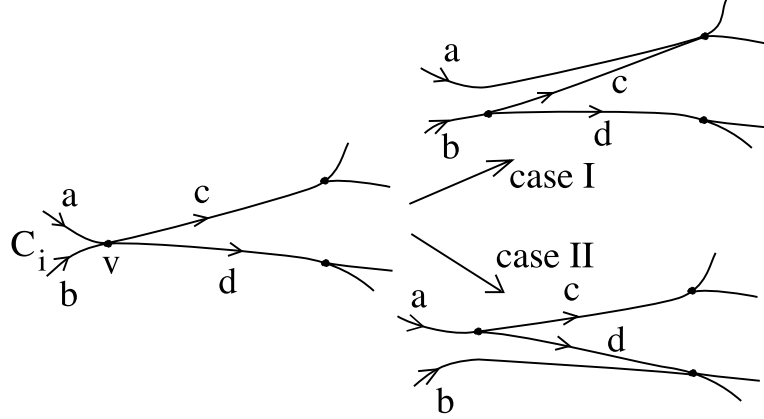
Figure 5: The splitting morphisms.
