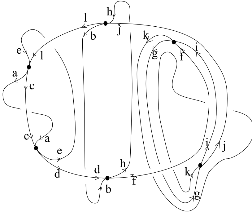
Figure 9: The Dehn twist T(i, g) .
