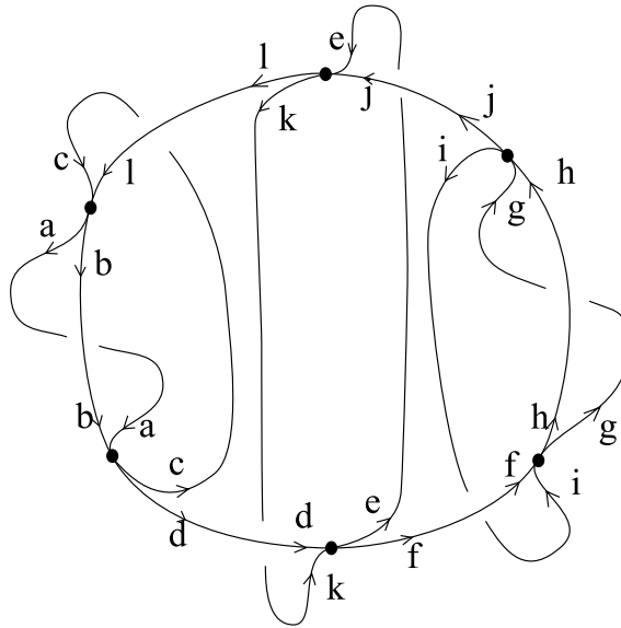
Figure 6: The initial labelled train-track.
