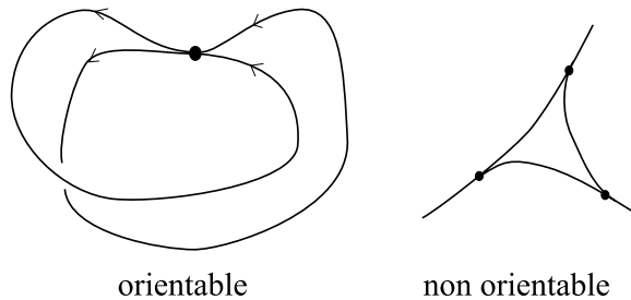
Figure 3: Orientable and non orientable train tracks.
