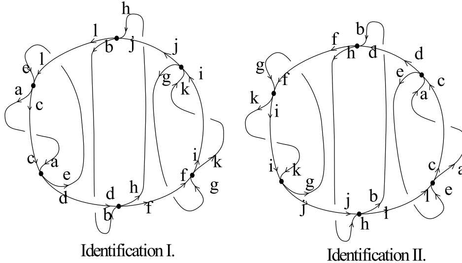
Figure 8: The two possible labelings.
