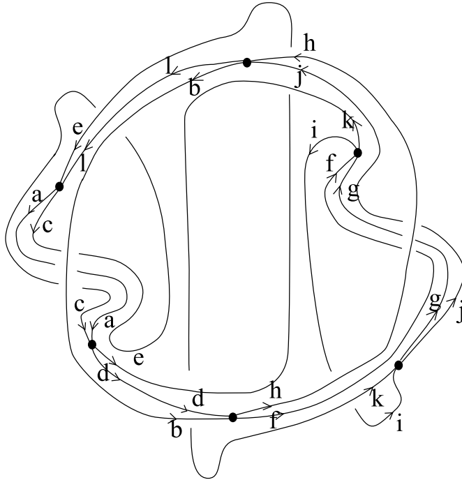
Figure 7: The image train track, after the sequence \mathcal{S}_1 of splittings, in the regular neighborhood of \tau .
