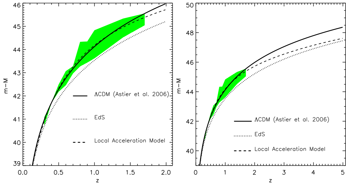
Figure 2. Left : the SNIa distance modulus is shown as a function of redshift for different cosmic expansion models: the best fitting \Lambda CDM model obtained by using distant supernovae [11] (solid), a decelerating Einstein deSitter model (dotted) and a model in which a large scale peculiar acceleration field acts on top of the EdS world model (short-dashed curves). The shaded area shows the state-of-the-art dispersion in the observed SNIa samples from the SNLS collaboration [10] and from the HST gold sample [11]. Right : We show the convergence, at high redshift, of the peculiar acceleration model to the underlying background cosmological model (an Einstein de Sitter model in this case).
