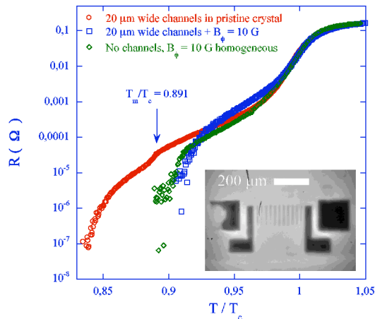
Figure 2. Resistance vs. temperature in H = 93 Oe, for the three \text{Bi}_2\text{Sr}_2\text{CaCu}_2\text{O}_8 crystals. The inset shows a magneto-optical image of the central part of crystal # 2, taken at T = 35 K and an applied field H = 456 Oe. The bright areas correspond to those parts of the crystal that are permeated by vortices, the dark zones are the irradiated areas that screen the field.
