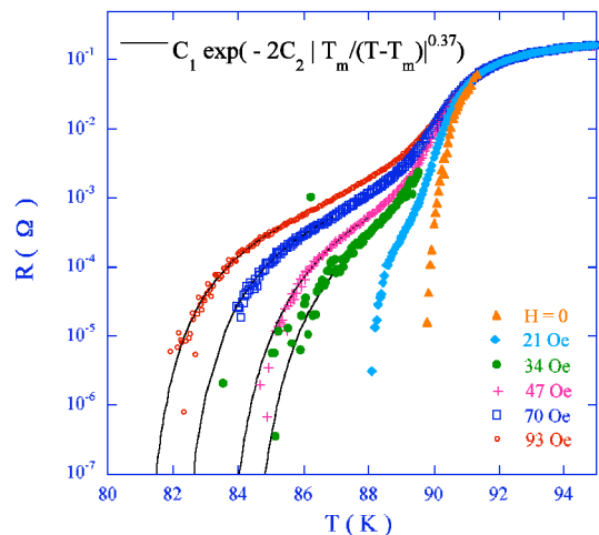
Figure 3. Resistivity vs. temperature for crystal # 2 ( 20 \mu\text{m} -wide channels in crystal with B_\phi = 10 G), for different values of the applied magnetic field. Drawn lines represent fits to Eq. (1).
